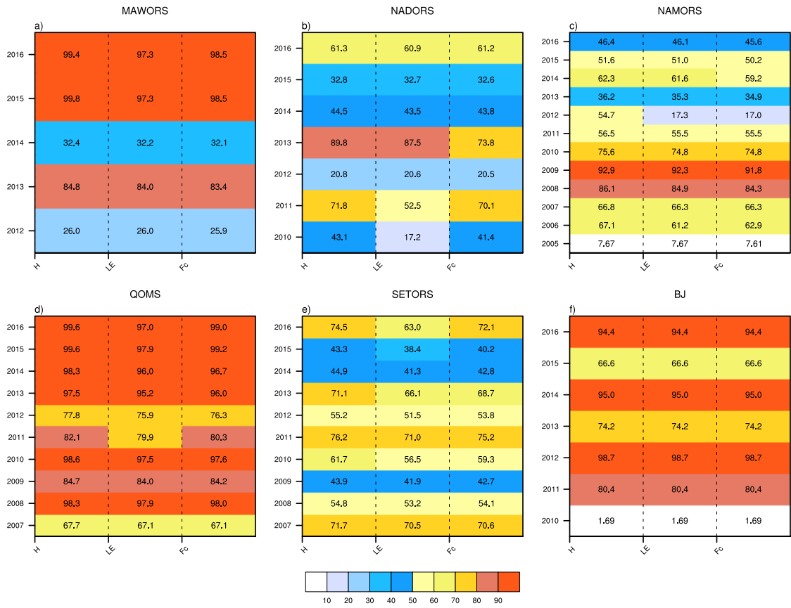
Figure A4. Same as Figure A1, but for the turbulent flux observations. H represents sensible heat flux and LE represents latent heat flux, and the CO 2 flux is expressed with Fc [Color figure can be viewed in the online issue].
