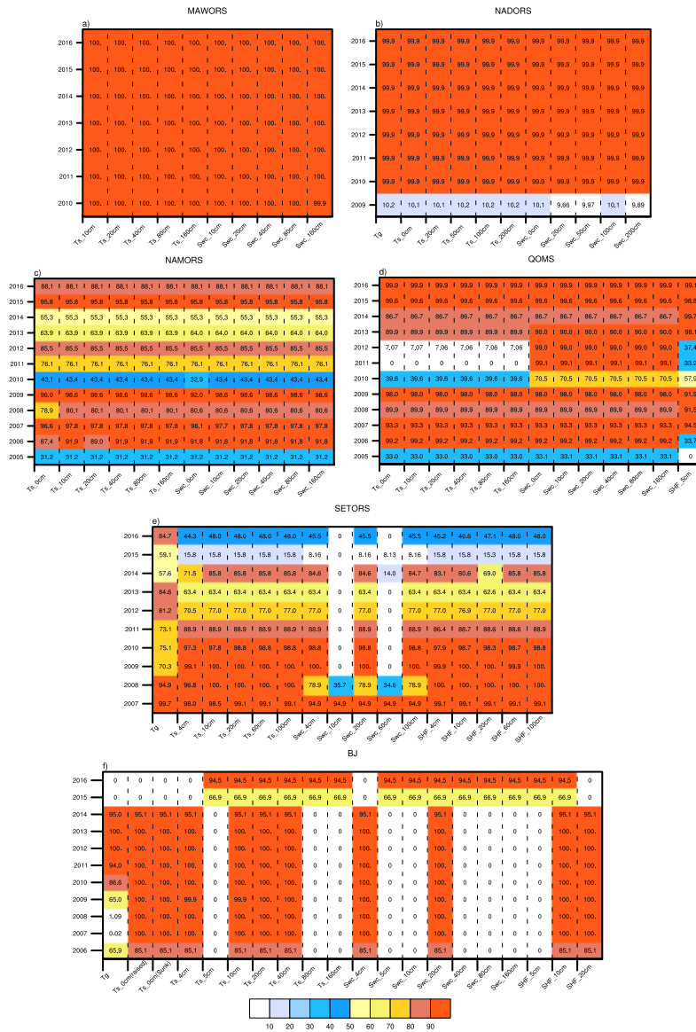
Figure A3. Same as Figure A1, but for the soil hydrothermal observations. Ground temperature is represented by Tg, and the soil temperature and soil water content are expressed with Ts and SWC, respectively; SHF refers to the soil heat flux [Color figure can be viewed in the online issue].
