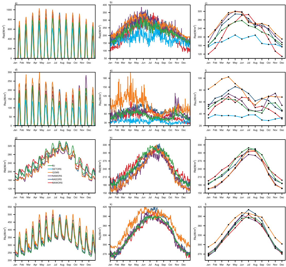
Figure 3. Same as Figure 2, but for the climatological average of the downward and upward solar radiation (Rsd and Rsu), and incoming and outgoing longwave radiation (Rld and Rlu), respectively [Color figure can be viewed in the online issue].
