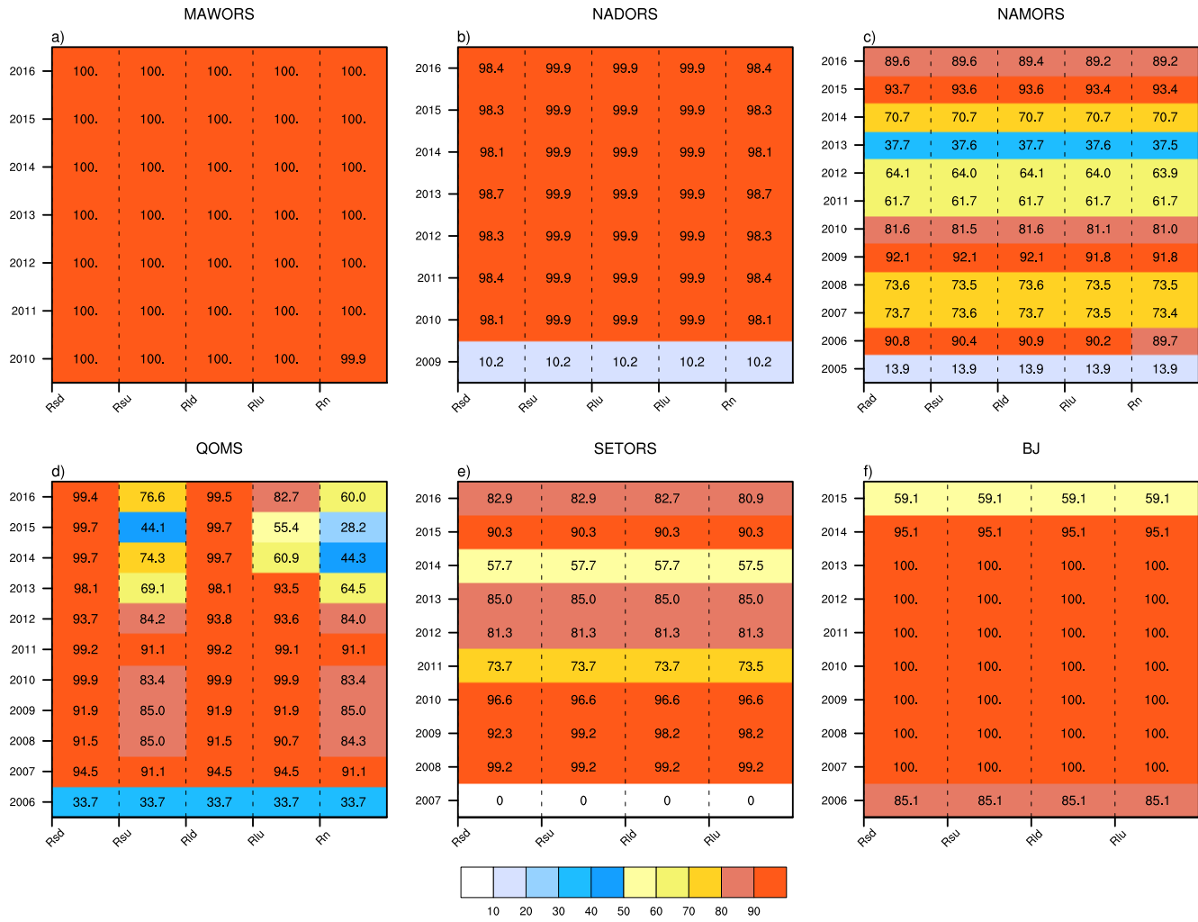
Figure A2. Same as Figure A1, but for the surface radiations. Rsd and Rsu represent the incoming and outgoing solar radiation, respectively; Rld and Rlu refer to the downward and upward longwave radiation. The net radiation is expressed using Rn [Color figure can be viewed in the online issue].
