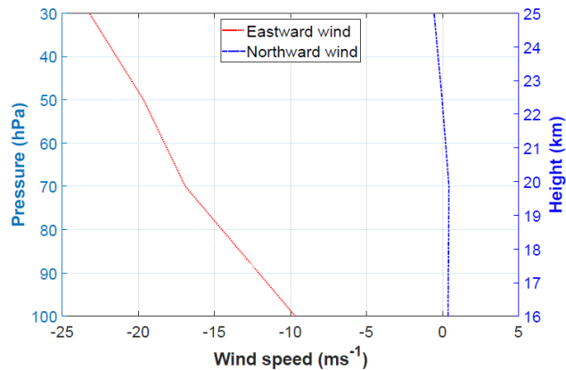
Figure S2: Mean lower stratosphere northward and eastward wind components for August 3 rd and 4 th 1991 in the latitude between 15 and 20 °N and the longitudes 60 to 40 °W using the NCEP Reanalysis data.
