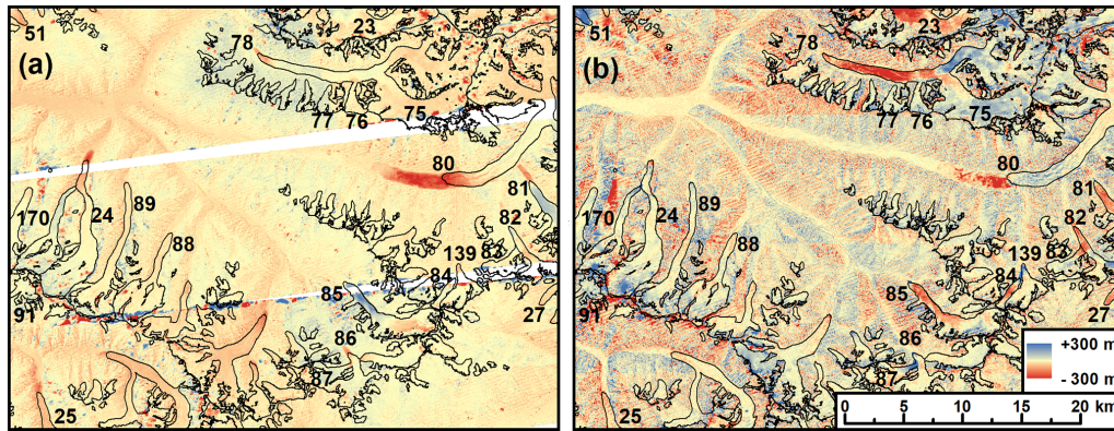
Figure 3. Two examples of colour-coded DEM difference images used to identify surging glaciers (marked with their ObjectID). The glacier outlines depict the glacier state in ~ 2000 (GI-2). (a) SRTM-Corona (2000–1968) and (b) AW3D30-SRTM (~ 2010–2000).
