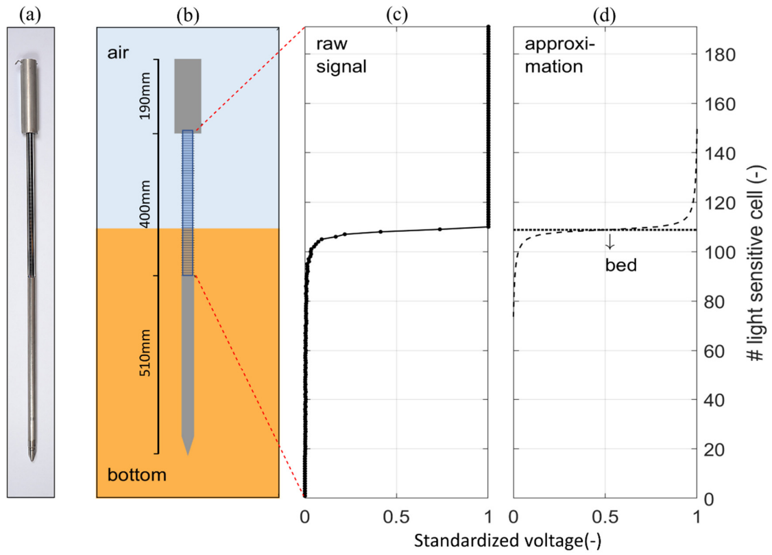
410 Figure 2. A photo (a) and schematization (b) of a SED-sensor in operation. The sensor uses an array of light-sensitive cells to determine the position of the bed level, resulting in a transection in the raw voltage output of the array (c). The noise in the raw signal is reduced, and the bed level is obtained by approximating the signal by an autonomous script (d). Details of SED-sensor data processing are included in Willemssen et al. (2018).
