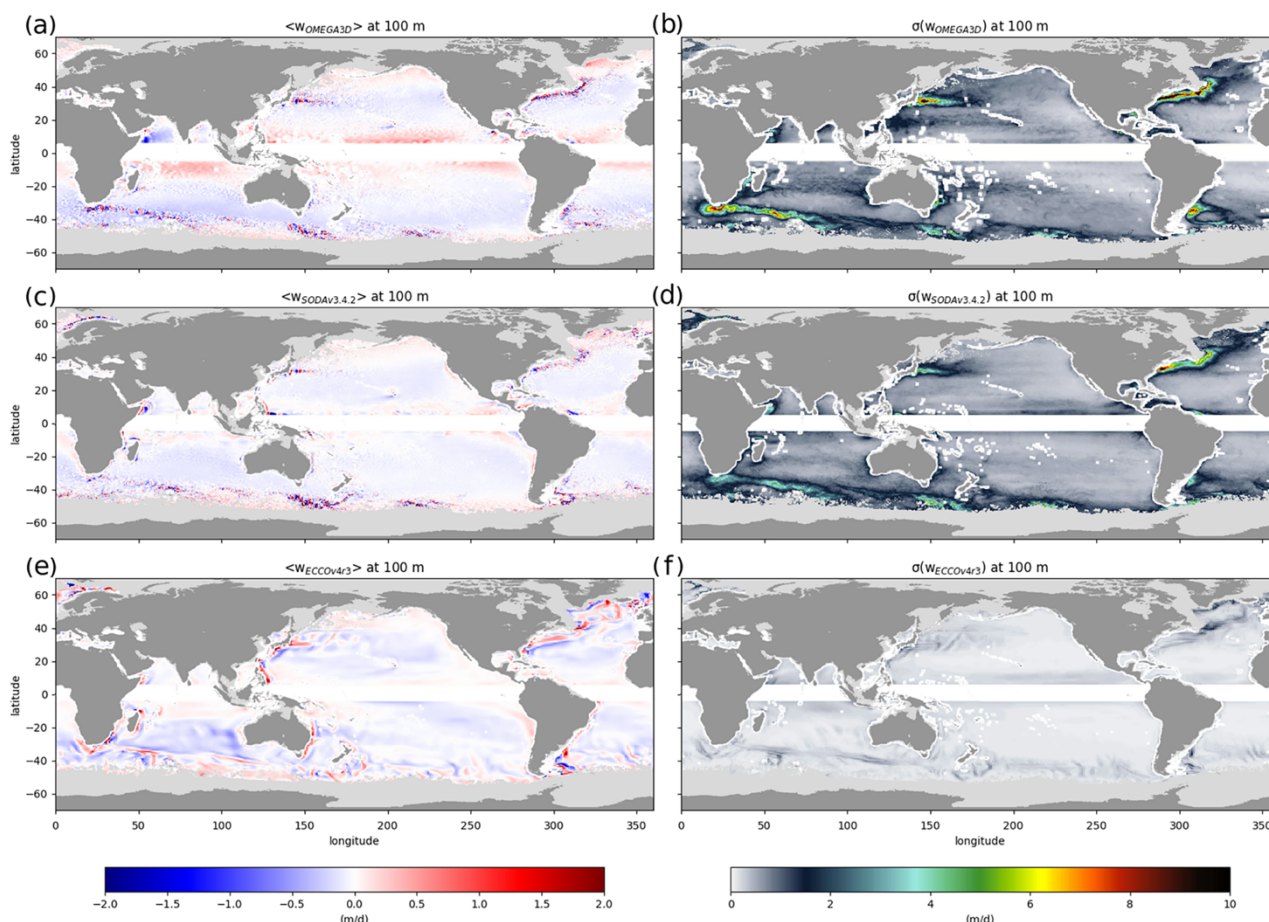
220 Figure 1. Mean vertical velocity at 100 m (a,c,e) and related standard deviation (b,d,f) computed from OMEGA3D (a,b), SODAv3.4.2 (c,d) and ECCOV4r3 (e,f) data on OMEGA3D domain over their 23 years overlapping period. Areas shallower than 100 m or contaminated at least once by sea-ice within the averaging period are masked in light grey.
