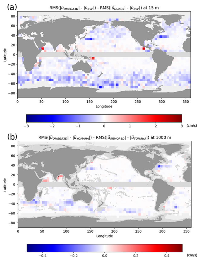
290 Figure 5. Difference between RMSD of OMEGA3D horizontal quasi-geostrophic and geostrophic velocities vs drifters in 5^\circ \times 5^\circ bins, at 15 m (a) and 1000 m (b) depth, respectively. Negative values indicate an improvement with respect to geostrophy.
