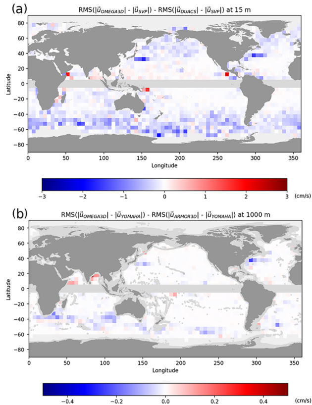
Figure 5. Difference between RMSD of OMEGA3D horizontal quasi-geostrophic and geostrophic velocities vs drifters in 5^\circ \times 5^\circ bins, at 15 m (a) and 1000 m (b) depth, respectively. Negative values indicate an improvement with respect to geostrophy.
