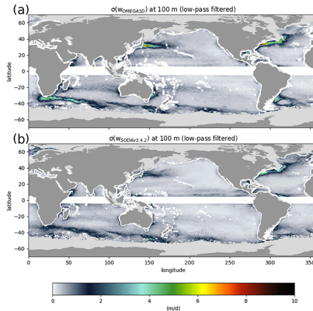
Figure 2. Mean monthly vertical velocity patterns and standard deviations computed from OMEGA3D (a), SODAv3.4.2 (b) after low-pass filtering the time series to remove signals above monthly frequency.
