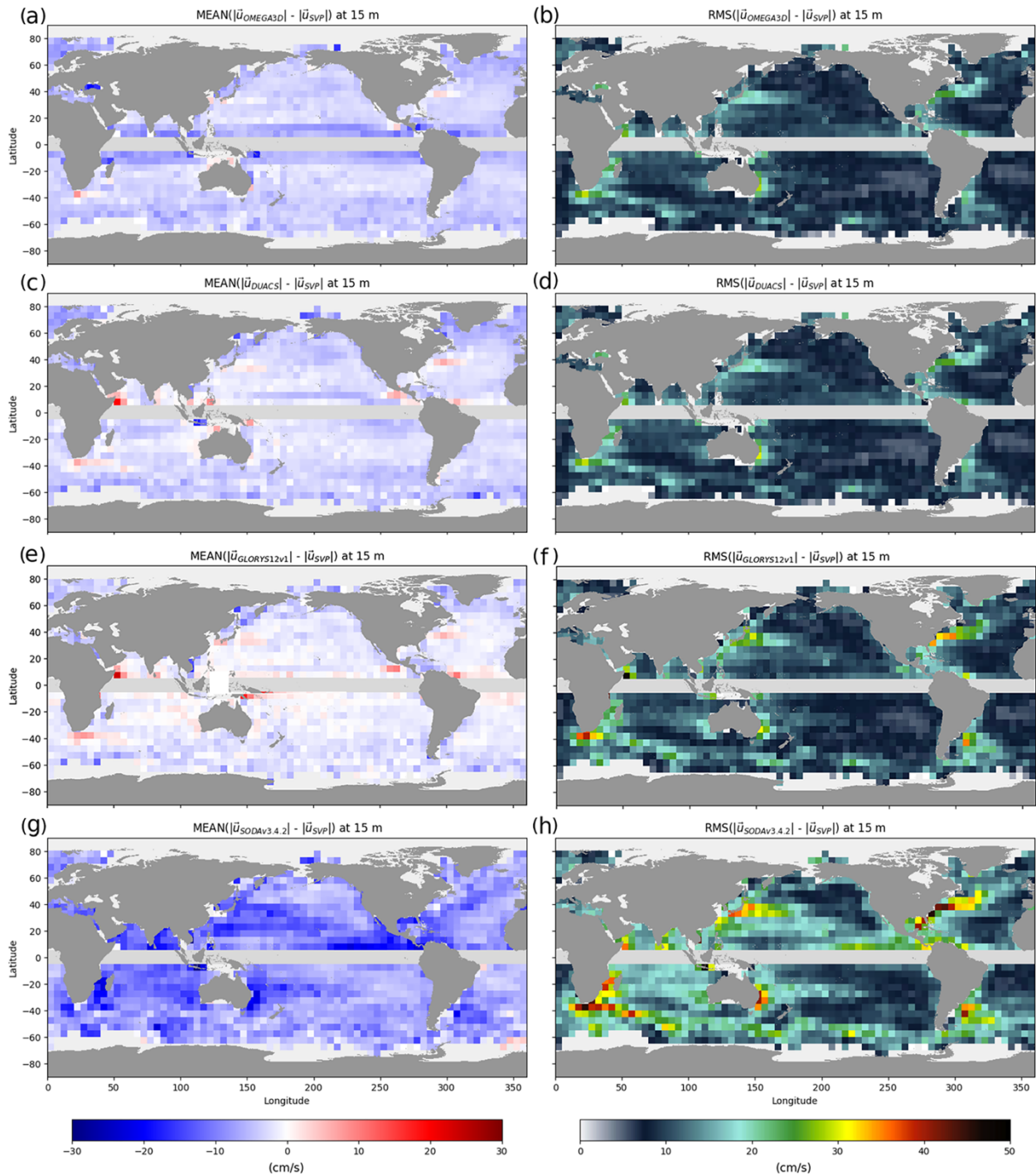
290 Figure 4: Mean and root mean square differences between OMEGA3D (a,b), DUACS (c,d), GLORYS12v1 (e,f), SODAv3.4.2 (g,h) velocities at 15 m depth and co-located SVP observations
