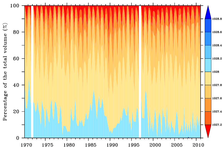
Figure 14. Volumetric potential density classes ranging from 1027.2 to 1028.8 \text{ kg.m}^{-3} in the Most Reliable Area between 1970–2010.
