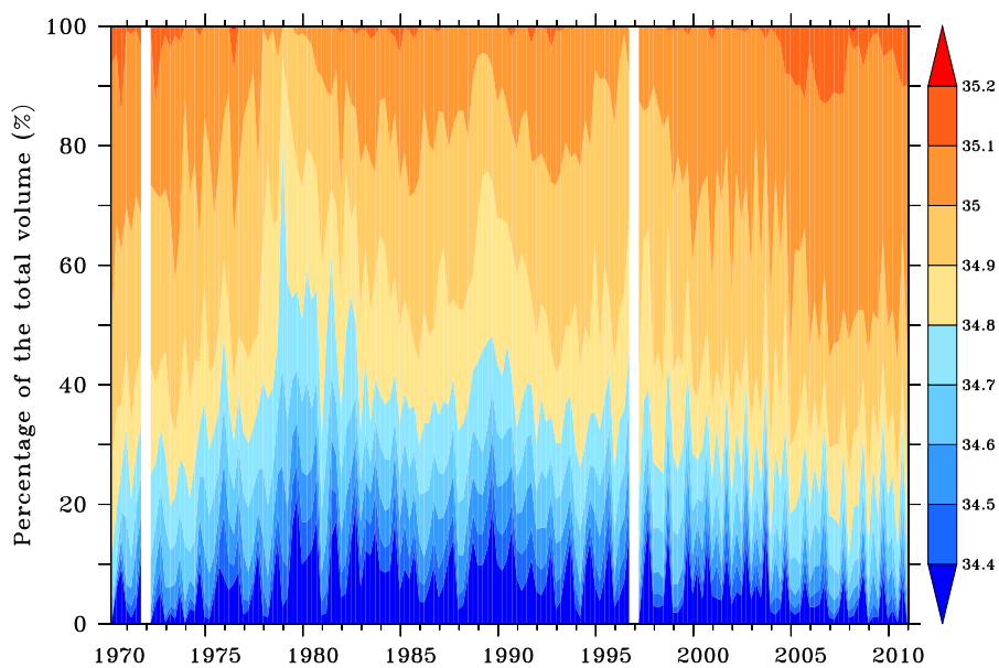
Figure 13. Volumetric salinity classes ranging from 34.4 to 35.2 PSU in the Most Reliable Area between 1970–2010.
