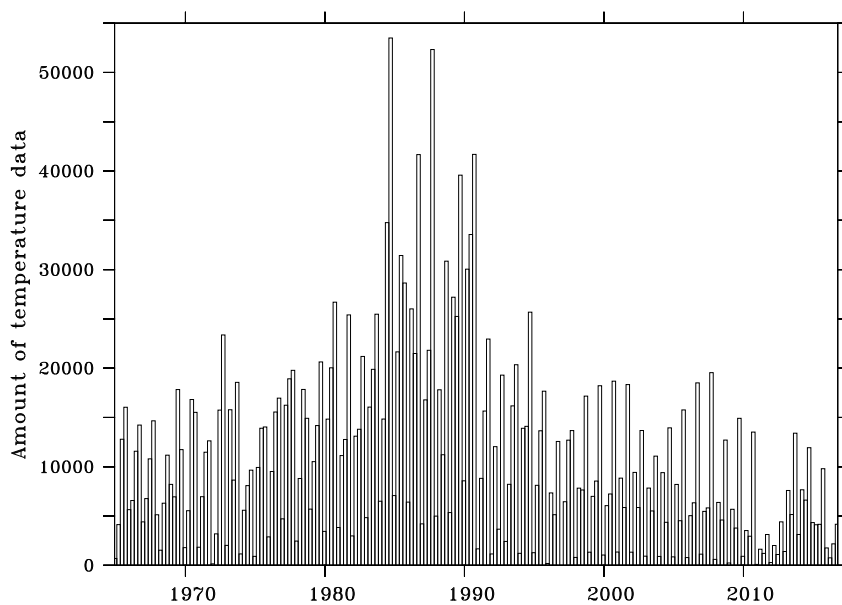
Figure 2. Availability of temperature data in the Barents Sea as a function of time.
