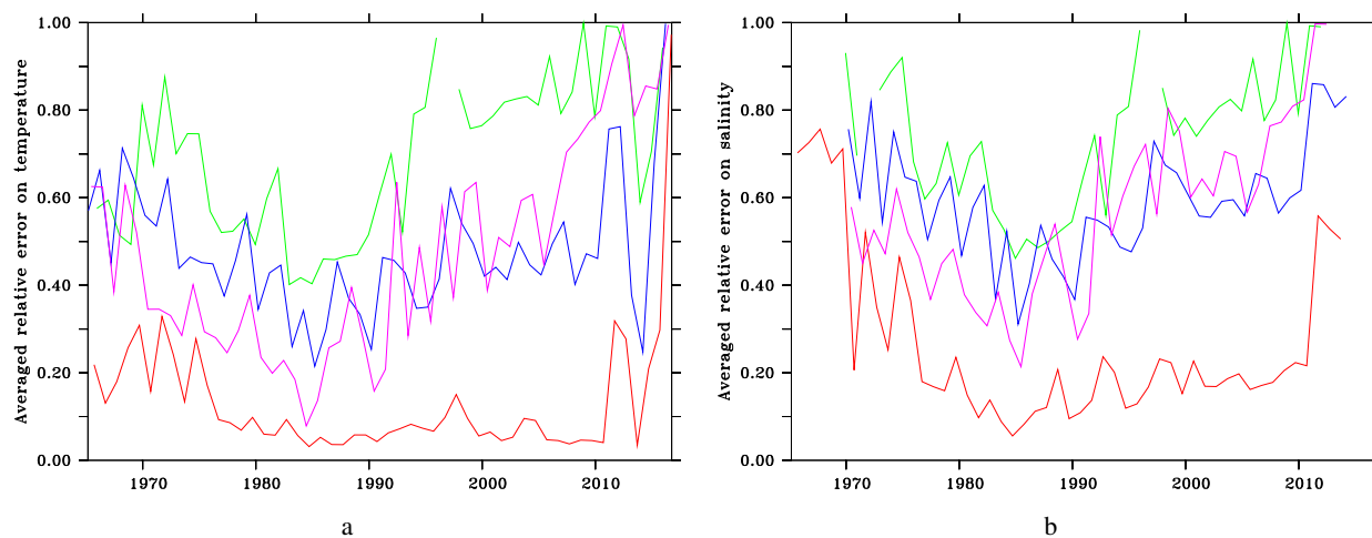
Figure 6. (a) Average relative error on the Barents Sea for temperature as a function of seasons: autumn (red), winter (green), spring (blue), summer (purple). (b) Average relative error on the Barents Sea for salinity.
