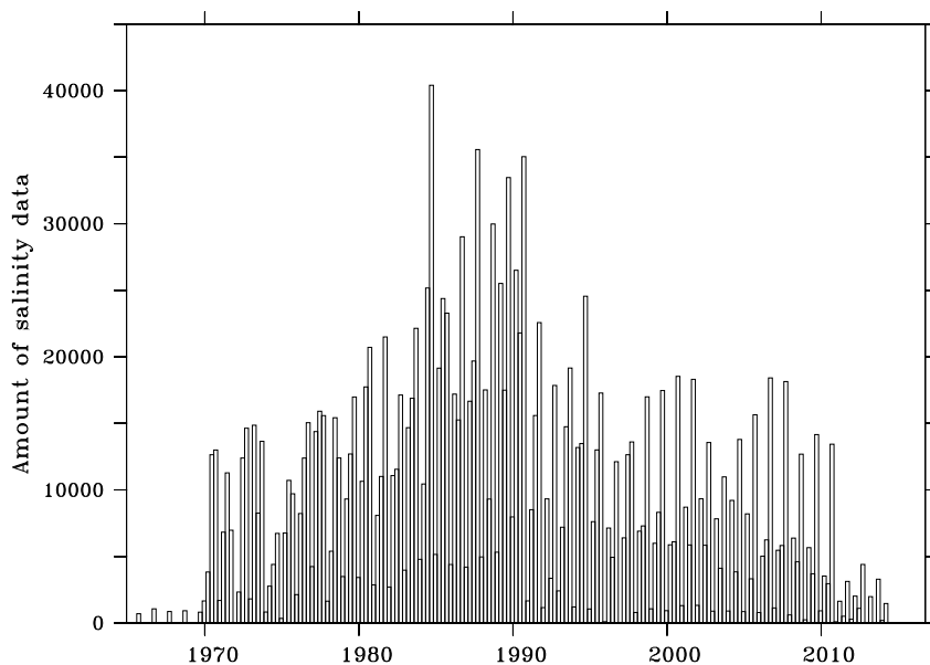
Figure 3. Availability of salinity data in the Barents Sea as a function of time.
