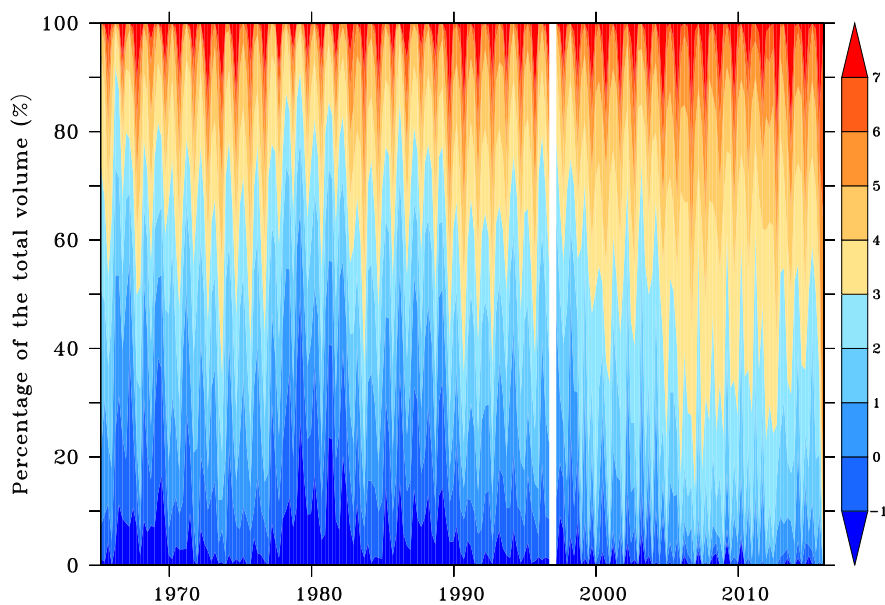
Figure 12. Volumetric temperature classes ranging from -1 to +7 °C in the Most Reliable Area between 1965–2015.
