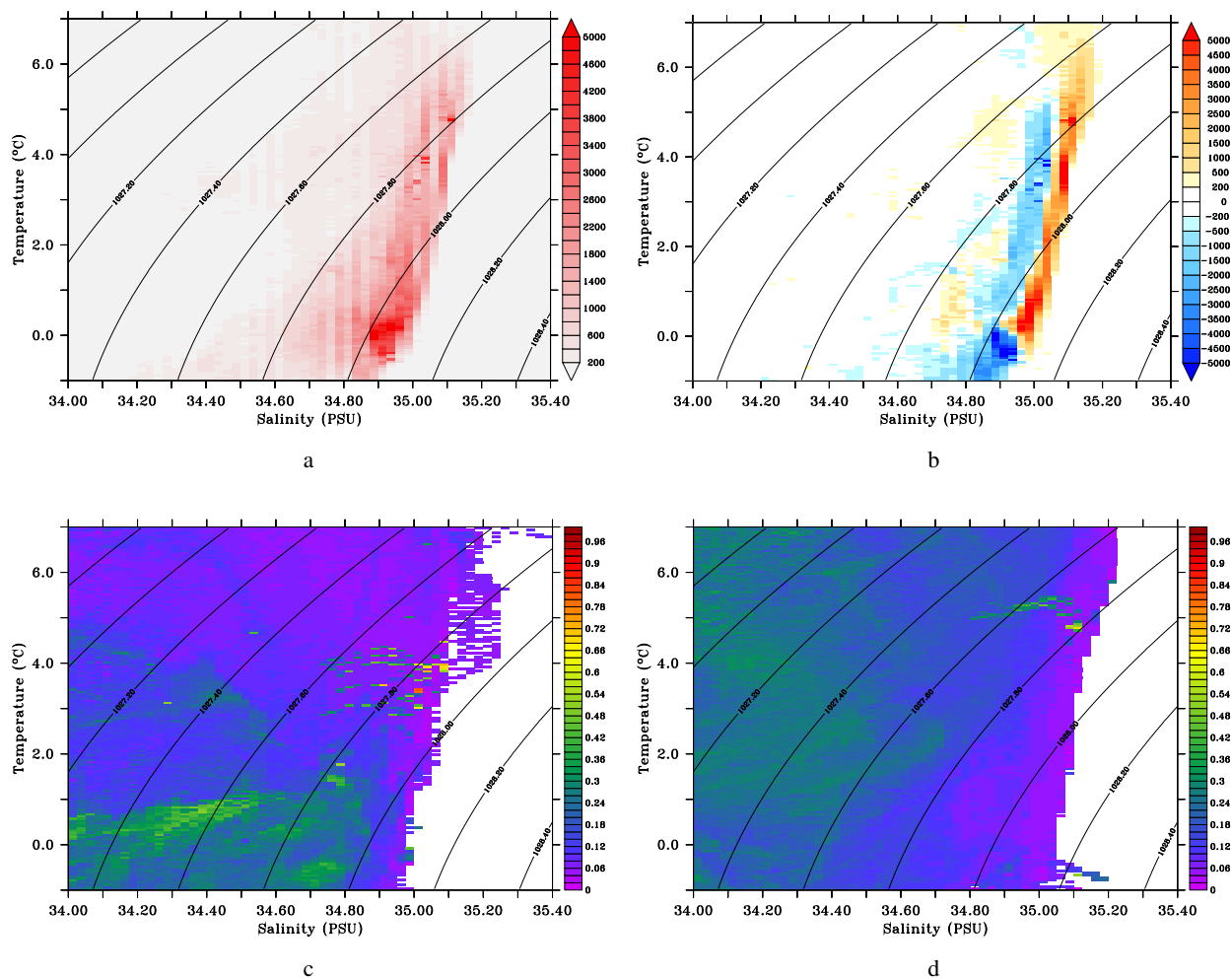
Figure 7. (a) Average volumetric T - S diagrams during 1994–1998 and 2006–2010. A value of 1 corresponds to a pixel with a vertical extent of 1 m. Isopycnals are shown for 0 m (black). (b) Difference in volumetric T - S diagrams between 2006–2010 and 1994–1998. (c) Average relative error weighted by the layer thickness for each T - S class between 1994–1998. (d) Average relative error weighted by the layer thickness for each T - S class between 2006–2010.
