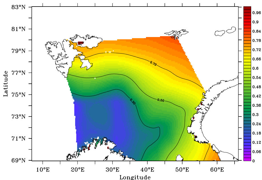
Figure 4. Average relative error at the Barents Sea surface for temperature between 1965–2015.
