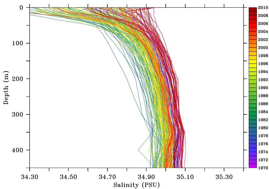
Figure 10. Seasonal averaged profiles of salinity on the Most Reliable Area between 1970–2010.
