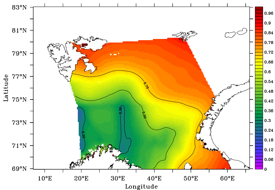
Figure 5. Average relative error at the Barents Sea surface for salinity between 1965–2015.
