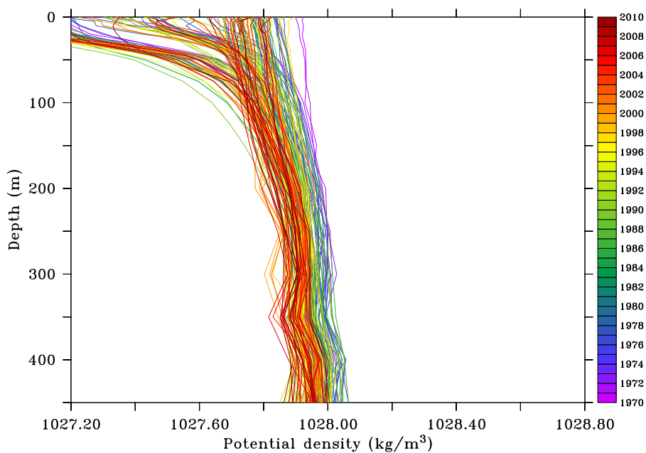
Figure 11. Seasonal averaged profiles of potential density on the Most Reliable Area between 1970–2010.
