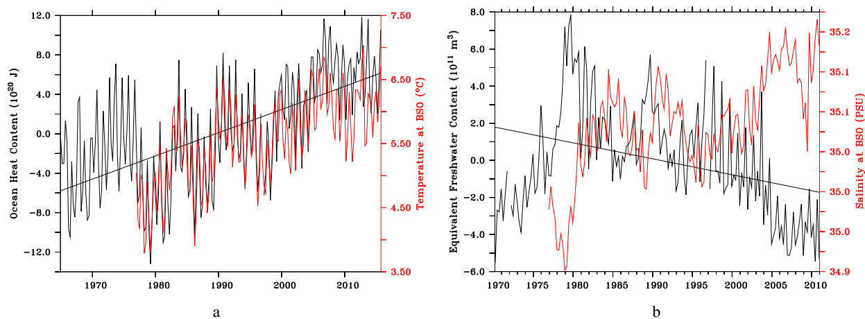
Figure 15. (a) Ocean heat content in the Most Reliable Area between 1965–2015, its linear trend (black) and temperature at the Barents Sea Opening. (b) Equivalent freshwater content in the Most Reliable Area between 1970–2010, its linear trend (black) and salinity at the Barents Sea Opening.
