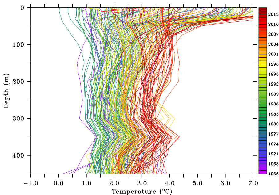
Figure 9. Seasonal averaged profiles of temperature on the Most Reliable Area between 1965–2015.
