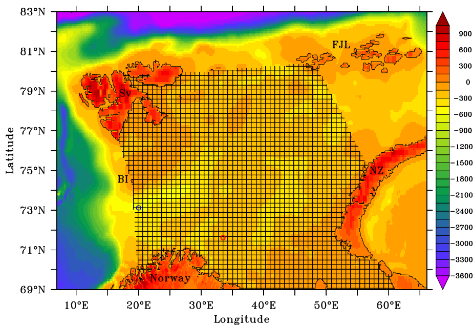
Figure 1. Bathymetry of the BS and its neighbouring seas. Our analyses on the Barents Sea correspond to the shaded region. The Barents Sea Opening, located between the Norwegian coast and Bear Island, and the Kola sections are shown as blue and red circles respectively. BI stands for Bear Island, Sv for Svalbard, FJL for Franz Jozef Land and NZ for Novaja Zemlja.
