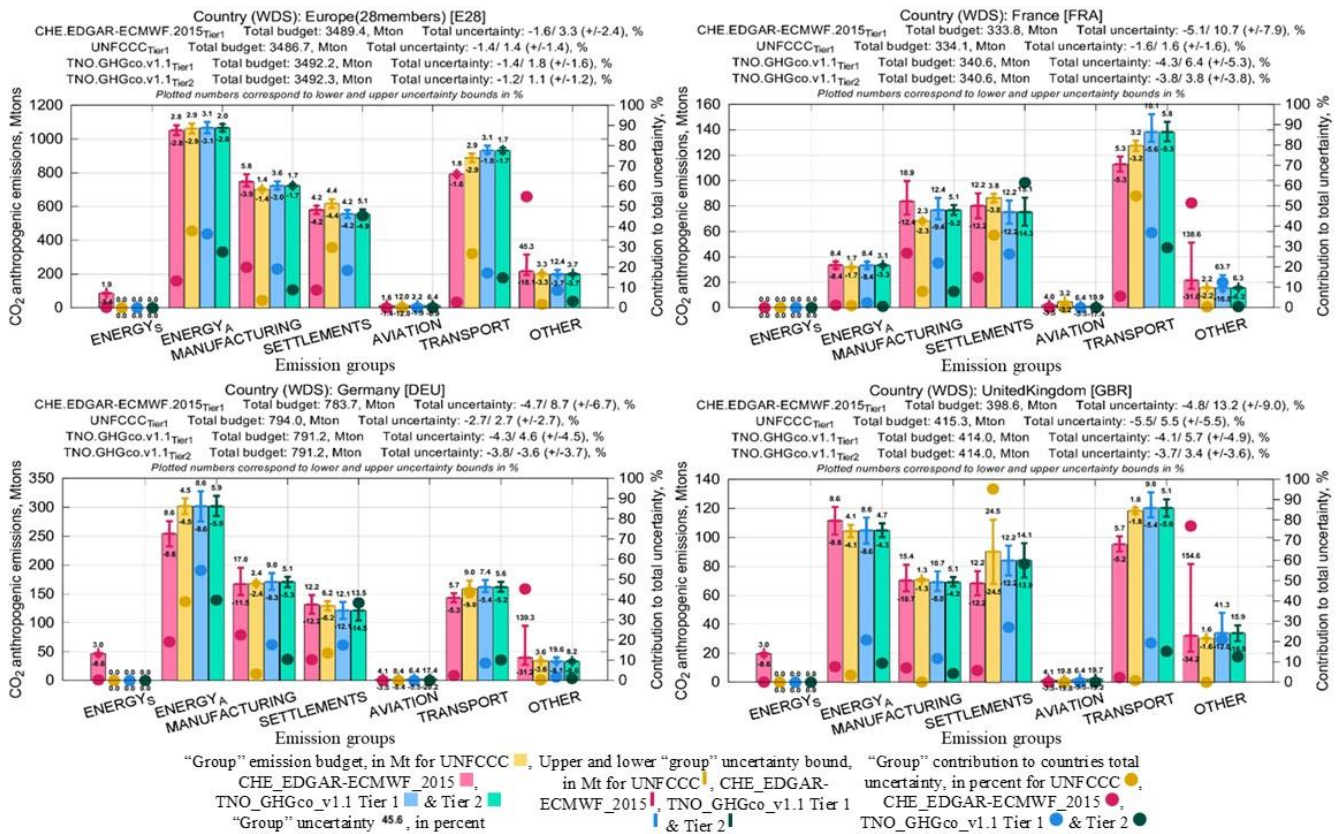
Figure 6: Emission budgets, uncertainties and contributions in percentage to the total uncertainty for Europe (E28), Germany (DEU), France (FRA) and United Kingdom (GBR)
