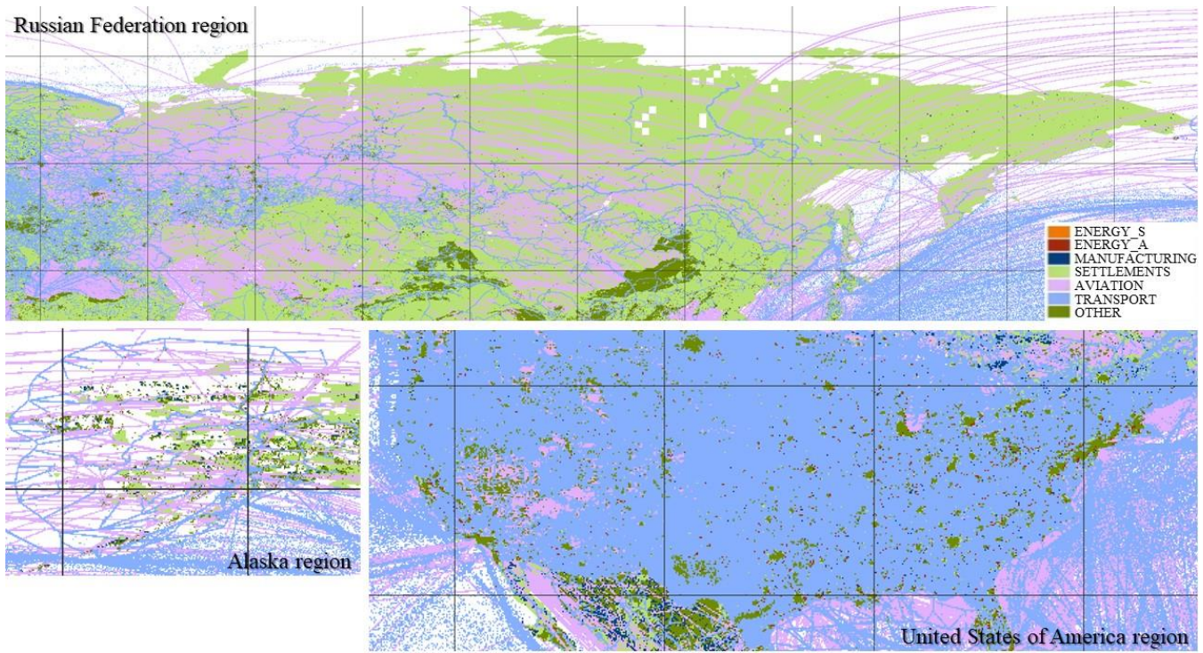
350 Figure 4c: Main emission “group” that contributes to the total uncertainty per grid-cell – the Russian Federation (top) and the United States of America (bottom) regions
