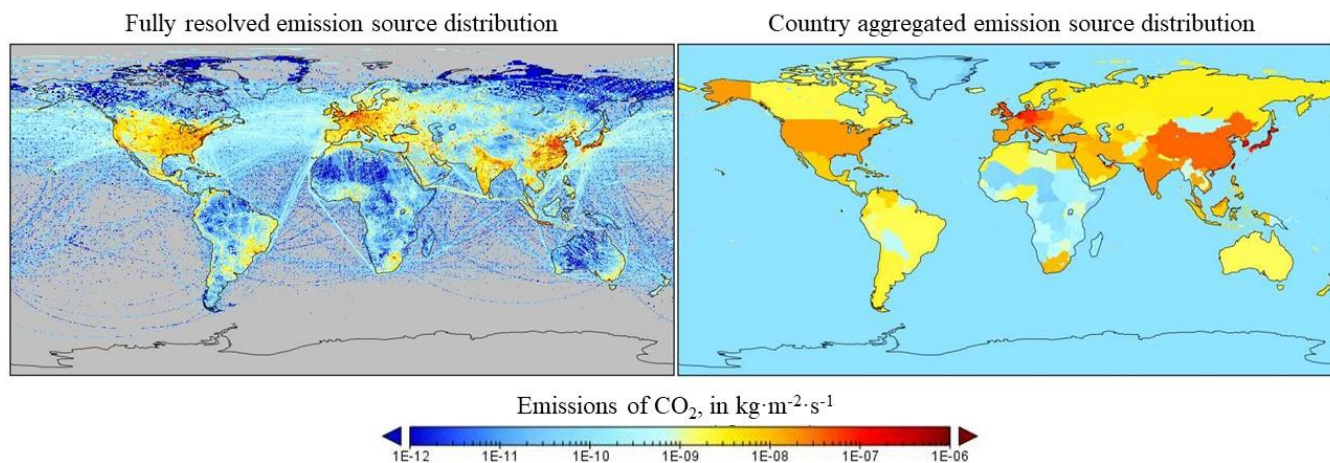
Figure 7: Anthropogenic CO 2 flux source distribution at ~25 km resolution – fully resolved (left), country aggregated (right)
