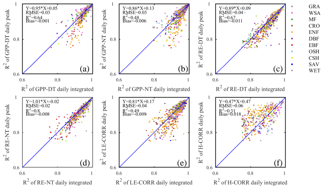
250 Figure 4: Comparison of the coefficients of determination ( R^2 ) of fitted seasonality curves between daily integrated fluxes (x-axis) and daily peak fluxes (y-axis) for GPP (a, b), RE (c, d), LE (e) and H (f). Both daytime (DT) and nighttime (NT) flux partitioning models are shown for GPP and RE.
