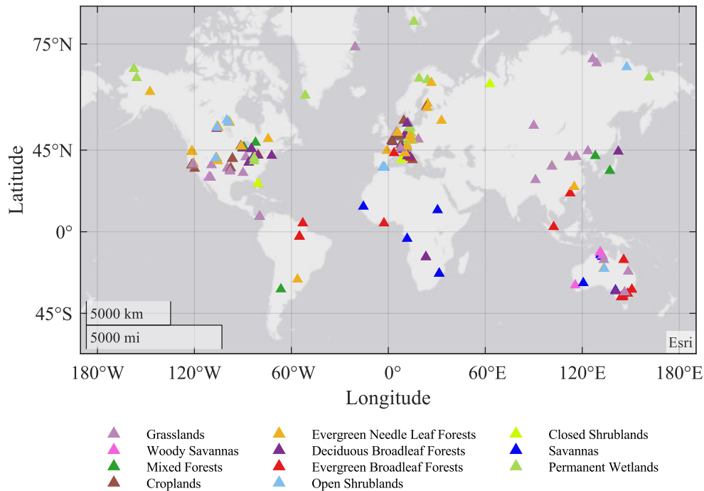
85 Figure 1: Global distribution of eddy covariance flux sites included in this study; color coded by their International Global Biosphere Programme (IGBP) biome classes.
