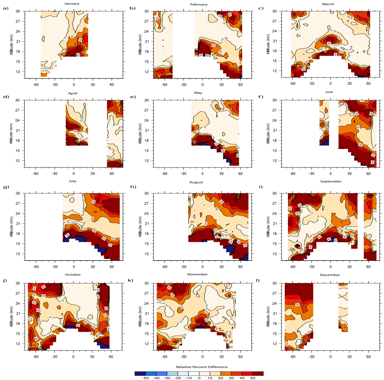
Figure 1. Altitude versus Latitude of relative percent difference of monthly climatology derived using OSIRIS 750 nm extinction and SAGEII/ SAGE III/ISS 525 nm extinction.
