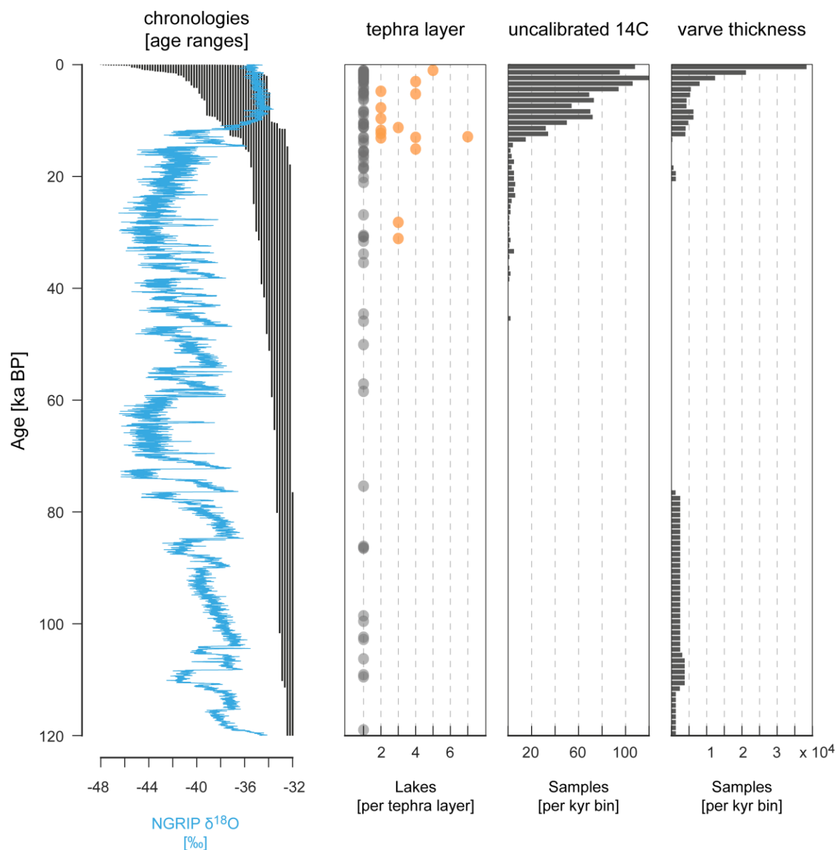
720 Figure 4: Temporal distribution of datasets in VARDA 1.0. a) Age range of chronologies indicated by black bars where each bar indicates the coverage of an individual chronology. The NGRIP stable oxygen record (Andersen et al., 2004) with the GICC05 chronology (Vinther et al., 2006; Rasmussen et al., 2006; Andersen et al., 2006; Svensson et al., 2005) is shown as a temporal reference curve. b) Tephra layers associated with lakes included in VARDA. Dots indicate the number of lakes associated with a single tephra layer. c) Number of samples per kyr bin of uncalibrated 14C measurements. d) Number of samples per kyr bin of individual varve 725 thickness measurements.
