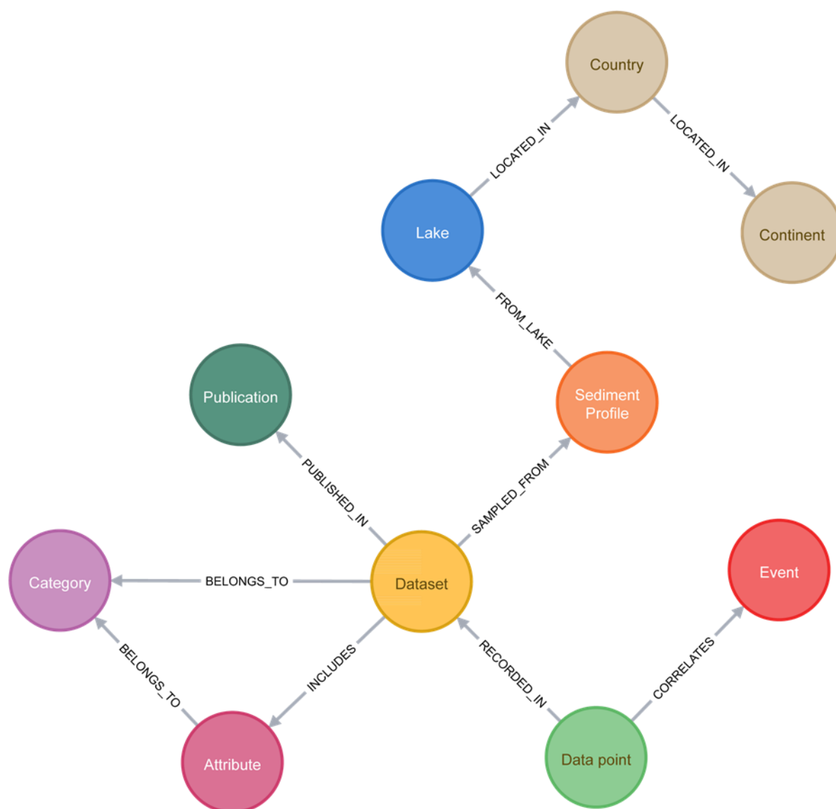
Figure 1: VARDA property graph model. Coloured circles represent nodes, grey arrows represent edges between nodes. For explanation see text.
