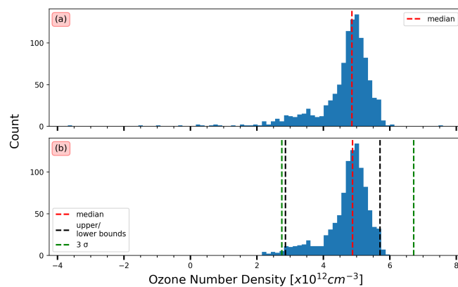
Figure 12. As Fig. 10 but for ozone data at 20 km between 65° and 75° S in December.
