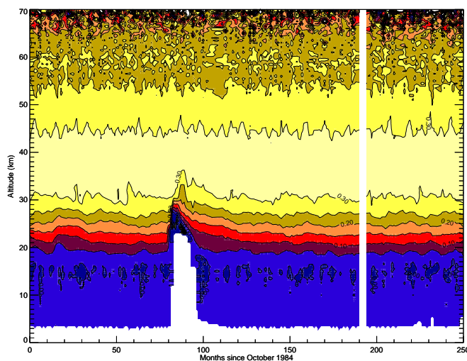
Figure 5. Measurement fraction, f , for 5^{\circ} N for all SAGE II data (no clearing) for the entire lifetime of the instrument. Note that the Mt Pinatubo period, particularly from month 81 (June 1991) to through roughly month 100 (the end of 1992) show clear reduction of the value of f above 18 km to as high as 35 km. Though several other volcanic events occur during the SAGE II lifetime (e.g. Ruiz/Nimuragya), none of these are readily apparent in f since they were an order of magnitude or more smaller than the Mt Pinatubo event.
