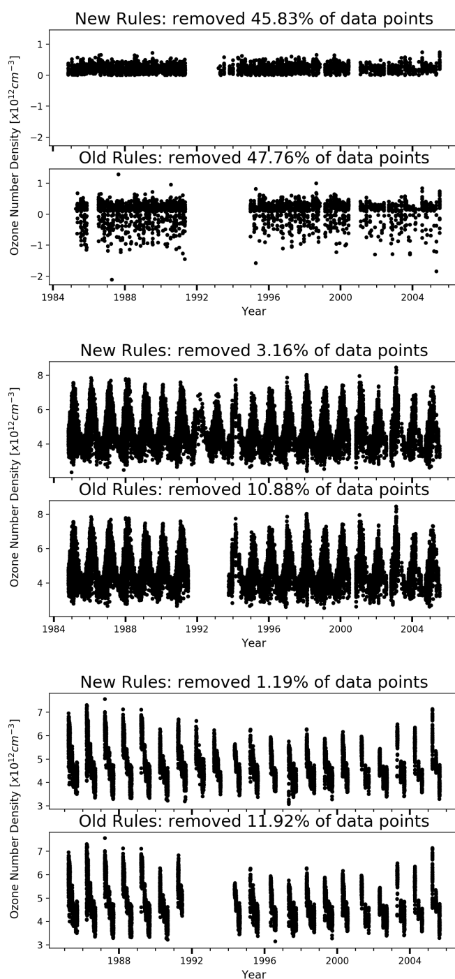
Figure 14. SAGE II ozone at: 16 km between 5° S and 5° N, 20 km between 45° and 55° N, and 20.5 km between 65° and 75° N. SAGE II data shown represent the remaining ozone data after the new (top) and current (bottom) rules were applied.
