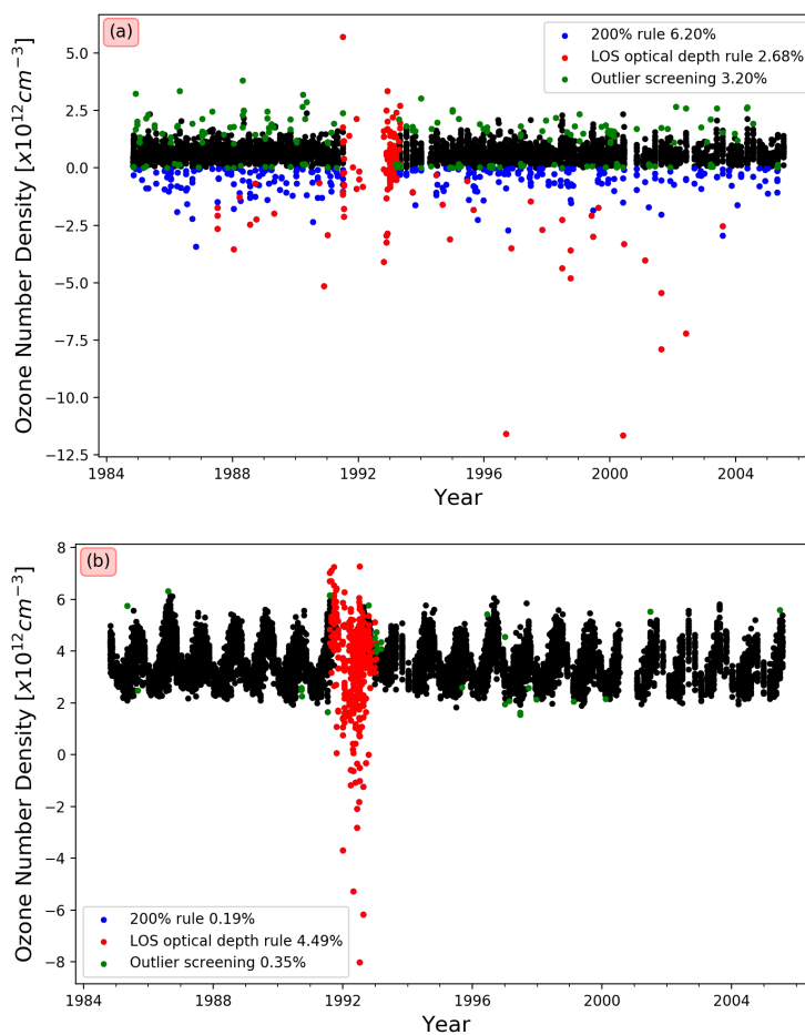
Figure 13. Number density ozone at 17 km between 15° and 25° N (a) and at 20.5 km between 25 and 35° S. The black dots represent the full SAGE II ozone data sets at the given altitude and latitude band, while the colored dots represent the ozone values that would be removed by applying the new rules (as indicated in the legend). Note that all rules were applied individually to all data points.
