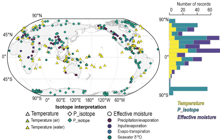
Figure 4. Left: Map of records in the Iso2k database with colours representing the first-order 'Isotope Interpretation' metadata field for each record (primary timeseries only; see Section 2.4). Symbols correspond to the three isotope interpretation 'supergroupings' (see Sections 4.3 and 5.1). Right: Bar chart showing the latitudinal distribution of records in the Iso2k database. Each bar represents ten degrees of latitude.
