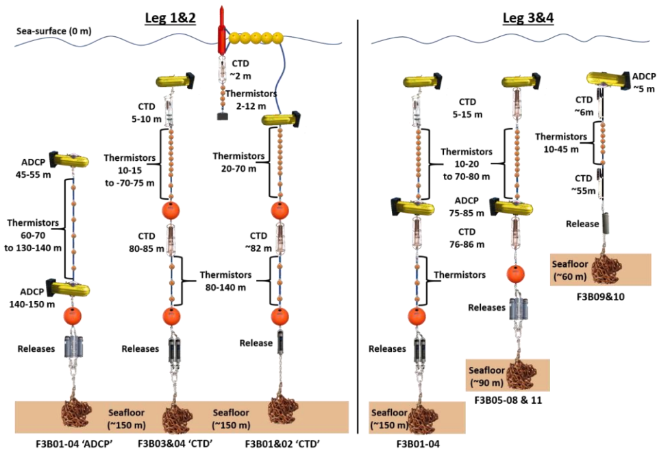
Figure 2: DFO taut line moorings, leg1&2 (left), leg 3&4 (right). In leg 2, F3B01&2 'CTD' lines were converted to F3B03&04's design due to failures of the sea-surface part. A 110 m rope, without thermistors, was added under the bottom CTD of F3B08 to be deployed
