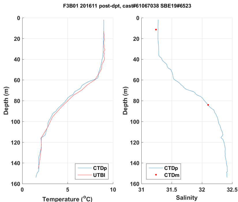
365 Figure 6: in-situ CTD profile (CTDp) comparison with moored thermistors (UTBI) and moored CTD (CTDm) on November 07 20 2016 at F3B01
