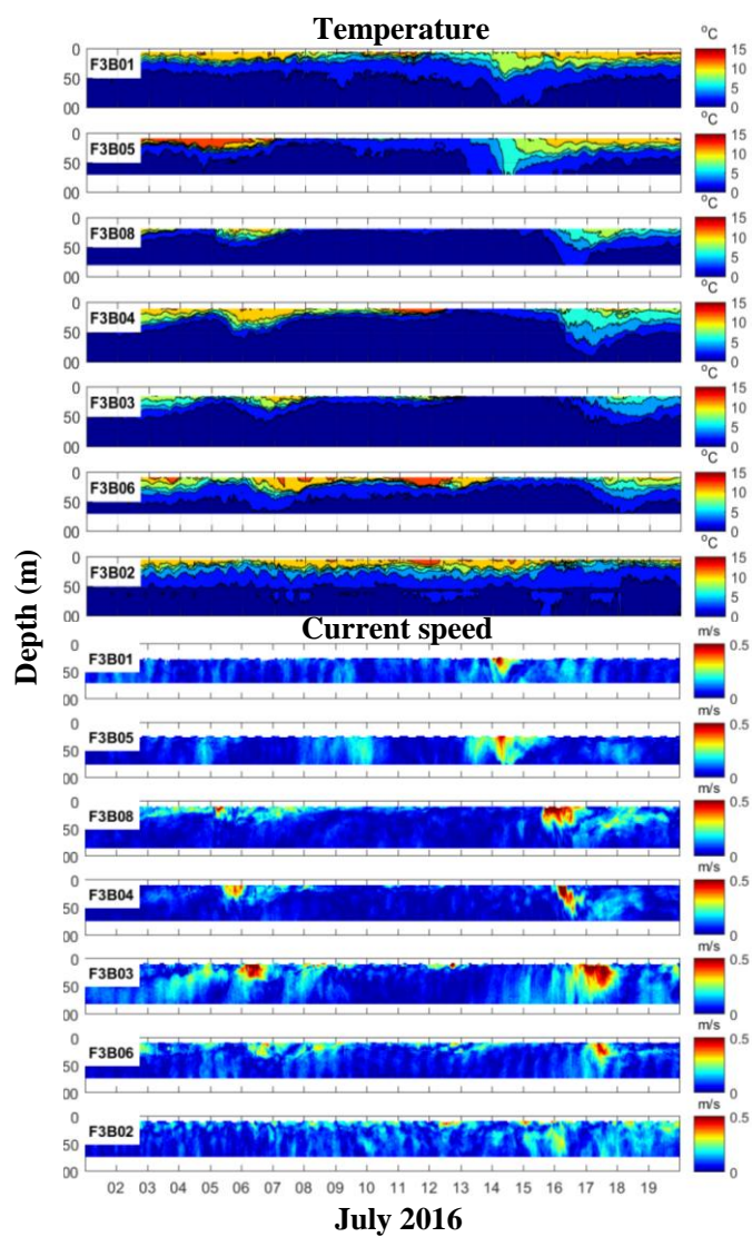
260 Figure 5: Fortune Bay water column thermal stratification and currents from July 1-20, 2016 showing several upwelling and downwelling events associated with strong currents 'pulses' travelling around the bay, i.e. from moorings F3B01 to F3B06.
