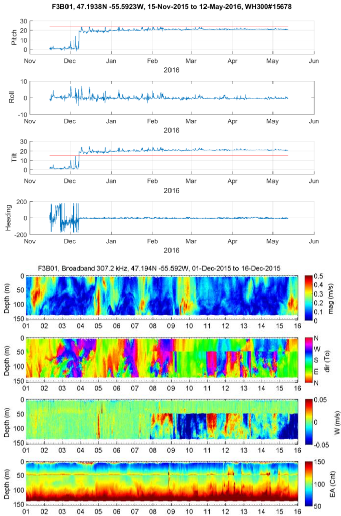
Figure 7: Example of an ADCP over-tilted issue. The event occurred on December 7, 2015 between 18:30 and 19:30, tilting the bottom ADCP of the mooring line on the pitch axis. Top four panels show the attitude sensor, pitch (1st panel), roll (2nd panel), calculated 'combined' tilt angle (3rd panel) and heading (4th panel) and as recorded by the instrument. Red lines on the pitch and tilt plots indicate the maximum sensor range as determined by bench test and the maximum accepted tilt angle of our quality control filter, respectively. The bottom four panels show current speed (mag), current direction (dir), current vertical component (w) and raw backscatter data (EA) zooming on the period 1-16 December 2015.
