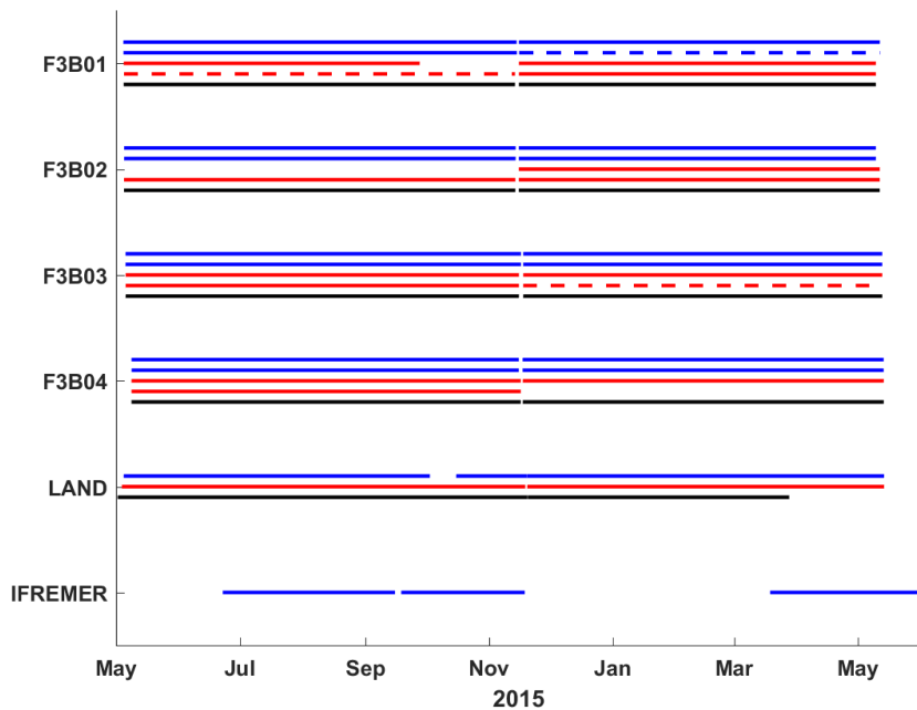
Figure 3: Data return, leg 1&2. For the moorings F3B01-04, ADCPs are in blue, CTDs are in red and UBTIs are in black. Top line correspond to the shallowest unit. For the land-based stations (LAND), DOGIS SUTRON weather station is in blue, DOGIS U30 weather station is in red and POOLC SUTRON tide gauge is in black. IFREMER ADCP data (SPMGF) is in blue. Dash lines represent partial data recovery (e.g. ADCP tilted, CTD having no or partial salinity return).
