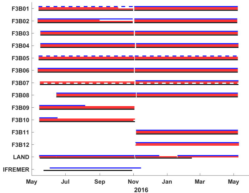
Figure 4: Data return leg 3&4. For the moorings F3B01-12, ADCPs are in blue, CTDs are in red and UBTIs are in black. Top line correspond to the shallowest unit. For the land-based stations (LAND), DOGIS SUTRON weather station is in blue, DOGIS U30 weather station is in red and POOLC SUTRON tide gauge is in black. IFREMER ADCP (SPMGF) and MASTODON (M01-12) data are in blue and black, respectively. Dash lines represent partial data recovery (e.g. ADCP tilted, CTD having no or partial salinity return).
