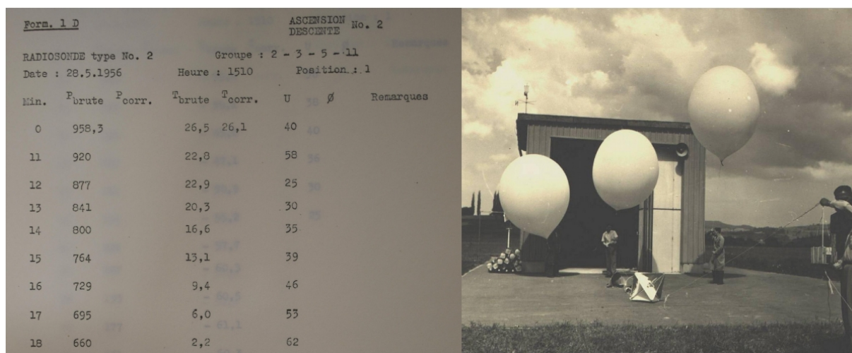
195 Figure 2: Left: Sounding data from the 1956 campaign held in Payerne, Switzerland, from the archive of MeteoSwiss in Payerne (own image). Right: At the beginning of the campaign, soundings were performed with four radiosondes on a train of balloons (archive of MeteoSwiss). Within the course of the campaign this procedure changed to 13 radiosondes on a train of several balloons.
