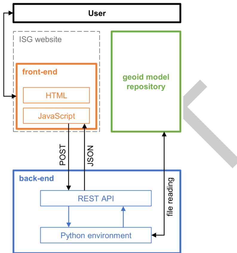
Figure 5. Logical structure of the height conversion web-service
