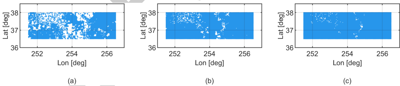
Figure 13. Agreement of local Colorado geoid model with respect to both global models: (a) residuals below 1\sigma ; (b) residuals below 2\sigma ; (c) residuals below 3\sigma are shown in blue
