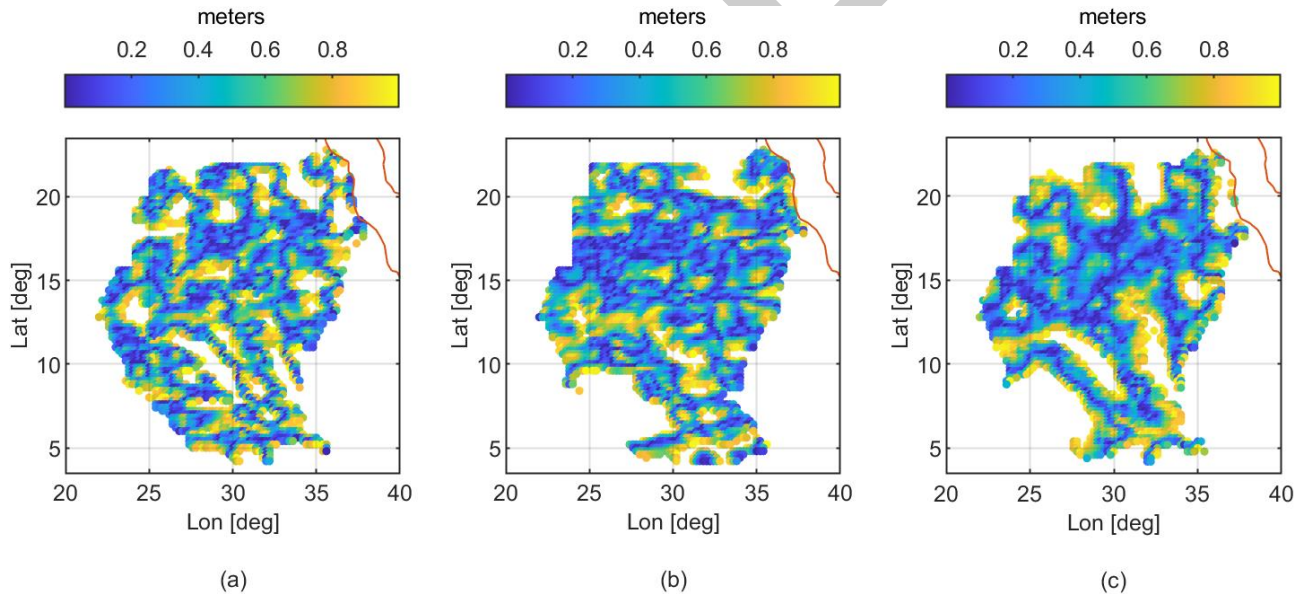
Figure 9. Sudanese geoids comparison, residuals with absolute value less than 1 meter. (a) case A; (b) case B; (c) case C.
