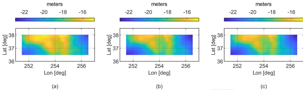
Figure 11. Local and global geoid models. The three panels show the undulation over the Colorado (US) area with respect to the reference ellipsoid of: (a) ColWLSC2020; (b) EIGEN-6C4; (c) EGM2008.
