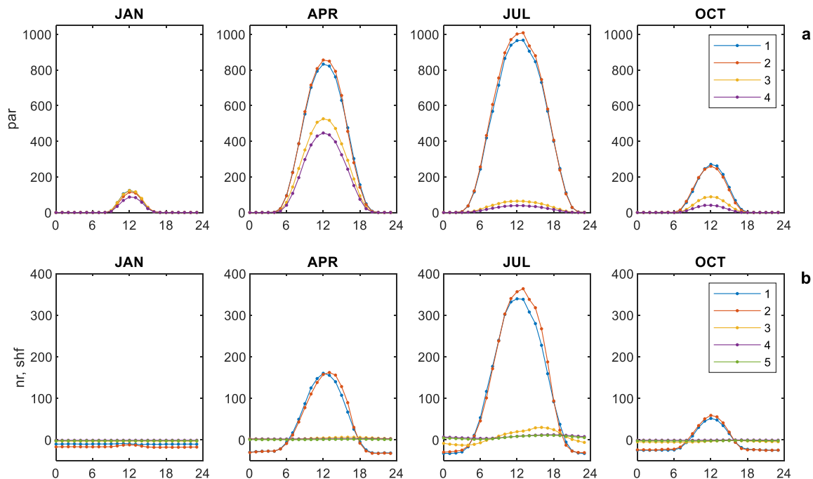
Figure 4. Monthly averaged diurnal course of incoming and reflected photosynthetically active radiation (a) ( \mu\text{mol m}^{-2} \text{s}^{-1} ) and net radiation balance, soil heat flux (b) ( \text{W m}^{-2} ) at hollow and ridge in January, April, July, and October. Mean values for 2010–2019. Legend: a) 1 – incoming PAR, hollow; 2 – incoming PAR, ridge; 3 – reflected PAR, hollow; 4 – reflected PAR, ridge. b) 1 – net radiation, hollow; 2 – net radiation, ridge; 3 – soil heat flux, hollow; 4 – soil heat flux, ridge, site 1; 5 – soil heat flux, ridge, site 2.
