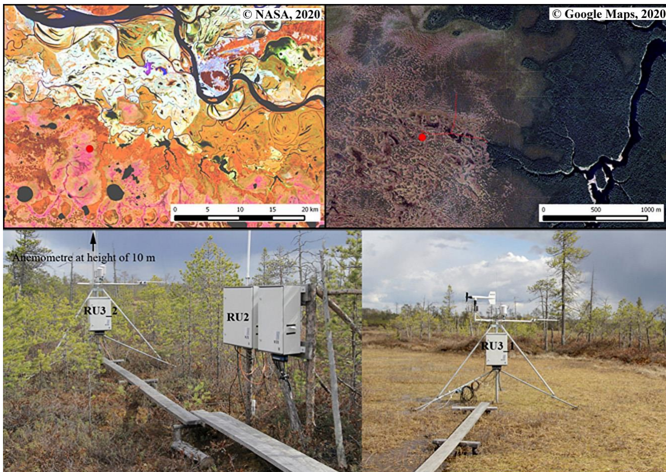
350 Figure 1. Position of the weather stations near Khanty-Mansiysk and among bog–forest landscapes (top panels © Landsat 7 ETM+ image, NASA, 2020; © Quickbird image, Google Maps, 2020). Automatic weather stations located at the treed ridge and the Sphagnum hollow (bottom panels Foto: Nina Filippova).
