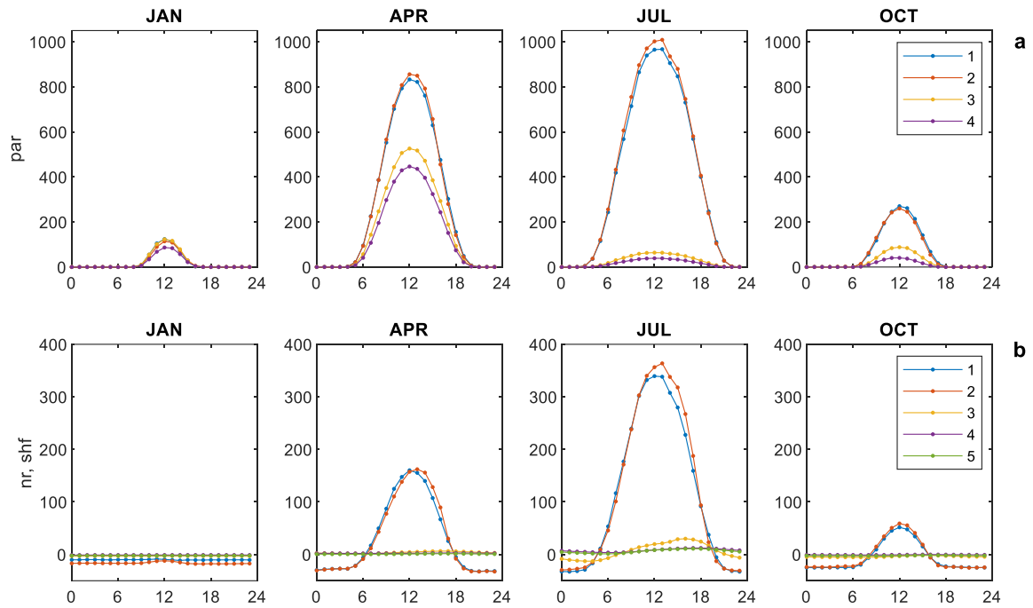
365 Figure 4. Monthly averaged diurnal course of incoming and reflected photosynthetically active radiation (a) ( \mu\text{mol m}^{-2} \text{s}^{-1} ) and net radiation balance, soil heat flux (b) ( \text{W m}^{-2} ) at hollow and ridge in January, April, July, and October. Mean values for 2010–2019. Legend: a) 1 – incoming PAR, hollow; 2 – incoming PAR, ridge; 3 – reflected PAR, hollow; 4 – reflected PAR, ridge. b) 1 – net radiation, hollow; 2 – net radiation, ridge; 3 – soil heat flux, hollow; 4 – soil heat flux, ridge, site 1; 5 – soil heat flux, ridge, site 2.
