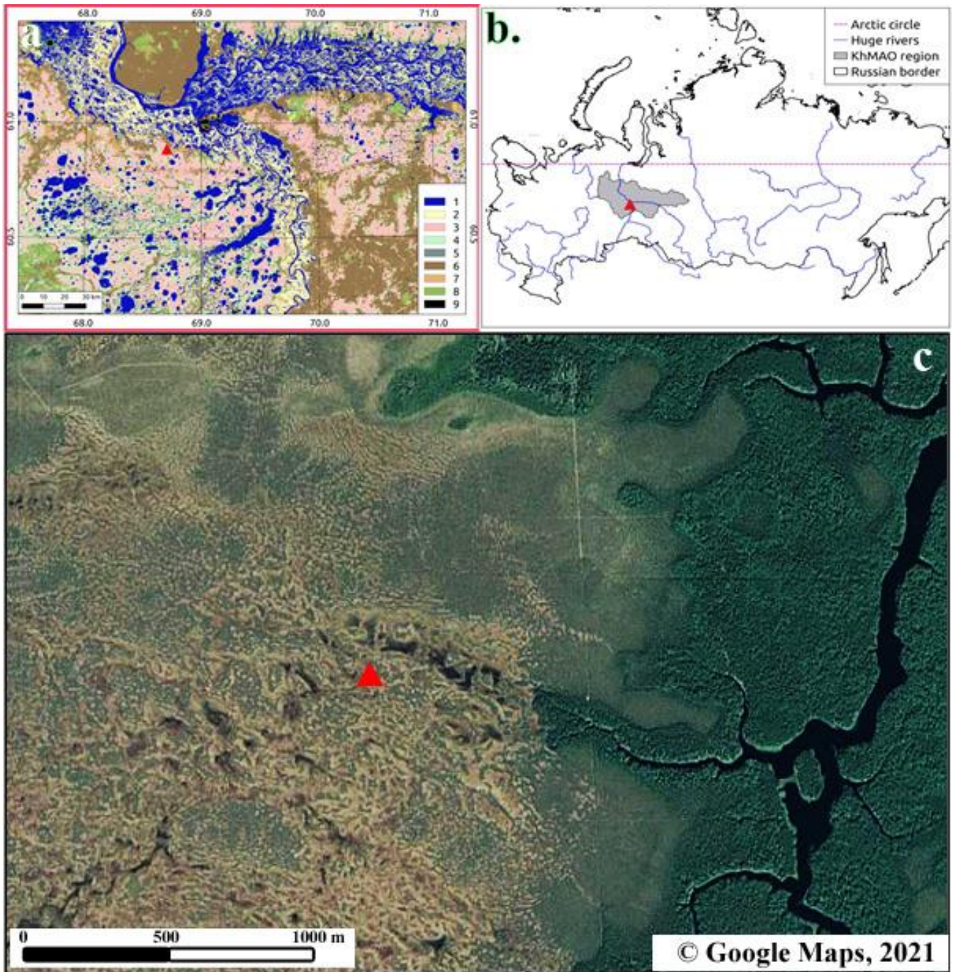
355 Figure 1. Position of the weather stations near Khanty-Mansiysk and among bog–forest landscapes. Top panel: (1 - water, 2 - floodplain, 3 - ridge-hollow bog, 4- ryam bog, 5 - pine forest, 6 - mixed forest, 7 - deciduous forest, 8 - burnt and disturbed forest, 9 – infrastructure. Bottom panel © Quickbird image, Google Maps, 2021.
