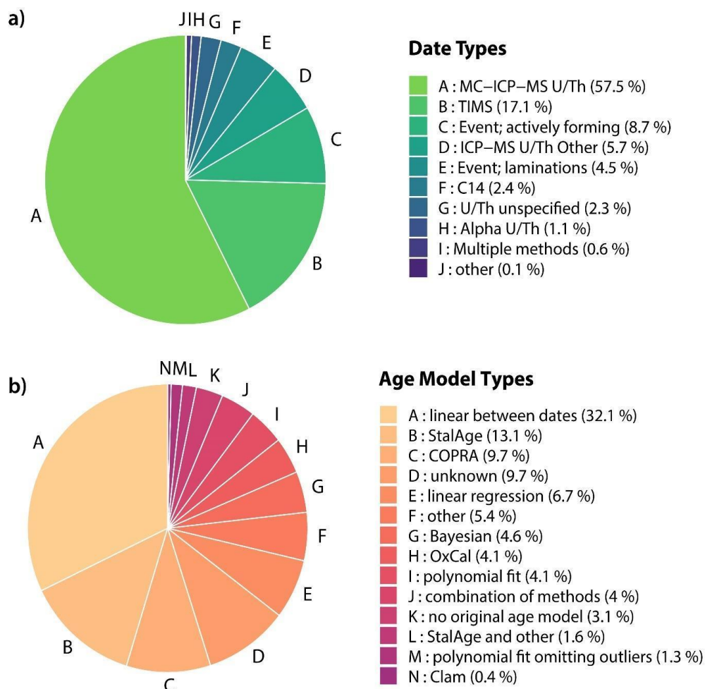
Figure 1: Summary of the dating information on which the original age-depth models are based (a) and the original age-depth model types (b) present in SISALv2.
