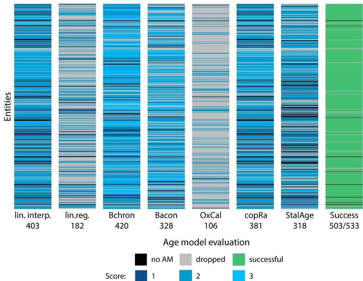
Figure 4: Visual summary of quality control of the automated SISAL chronology construction. The evaluation of the age-depth models for each method (x-axis) is given for each entity (y-axis) that was considered for the construction (n=533). Black lines mark age-depth models that could not be computed. Age-depth models dropped in the automated or expert evaluation are marked by grey lines. Age-depth models retained in SISALv2 are scored from 1 (only one criterion satisfied) to 3 (all criteria satisfied) in shades of blue. For 503 records alternative age-depth models with uncertainties are provided (green lines) in the “success” column.
