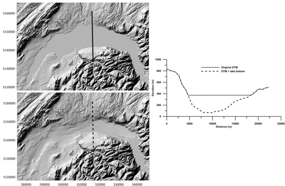
310 Figure 6: Examples of topography models used to calculate lake corrections (here, Lake Geneva, Switzerland). Top shaded relief represents the original DEM (MERIT), the bottom one the combination of DEM and lake bottom. The graph on the right shows two profile lines crossing both models (North is to the right).
