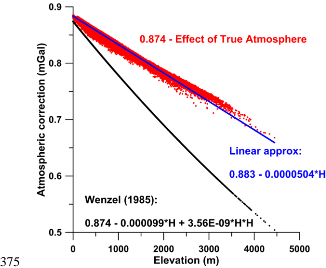
Figure 9: Comparison of atmospheric correction at selected points covering the whole AlpArray area. The black dots represent the atmospheric correction calculated by a simple approximation according to Wenzel (1985). The red dots show the calculation using the effect of true atmosphere subtracted from the global constant value of 0.874 mGal (Mikuška et al., 2008) and the blue line is its linear approximation.
