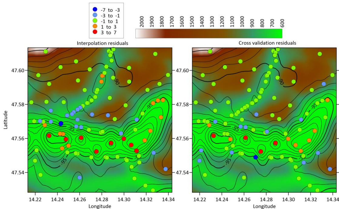
740 Figure 15: Interpolation and cross validation residuals of a subset within a small section of the Enns valley in Austria. Background: Topography, contour lines: CBA anomaly [mGal] interpolated using a high-resolution grid (about 200 m spacing), coloured dots: residuals (left: interpolation, right: cross validation) at the scattered data points with respect to the AlpArray CBA grid (2000 m spacing). Residuals in [mGal], height in [m].
