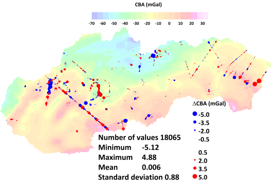
645 Figure 14: Differences between the CBA grid and independent gravity points (not used for the Slovakian part of the gravity grid compilation). It was calculated by SURFER's simple grid-residual procedure and showed that no gravity differences were greater than \pm 5 mGal.
