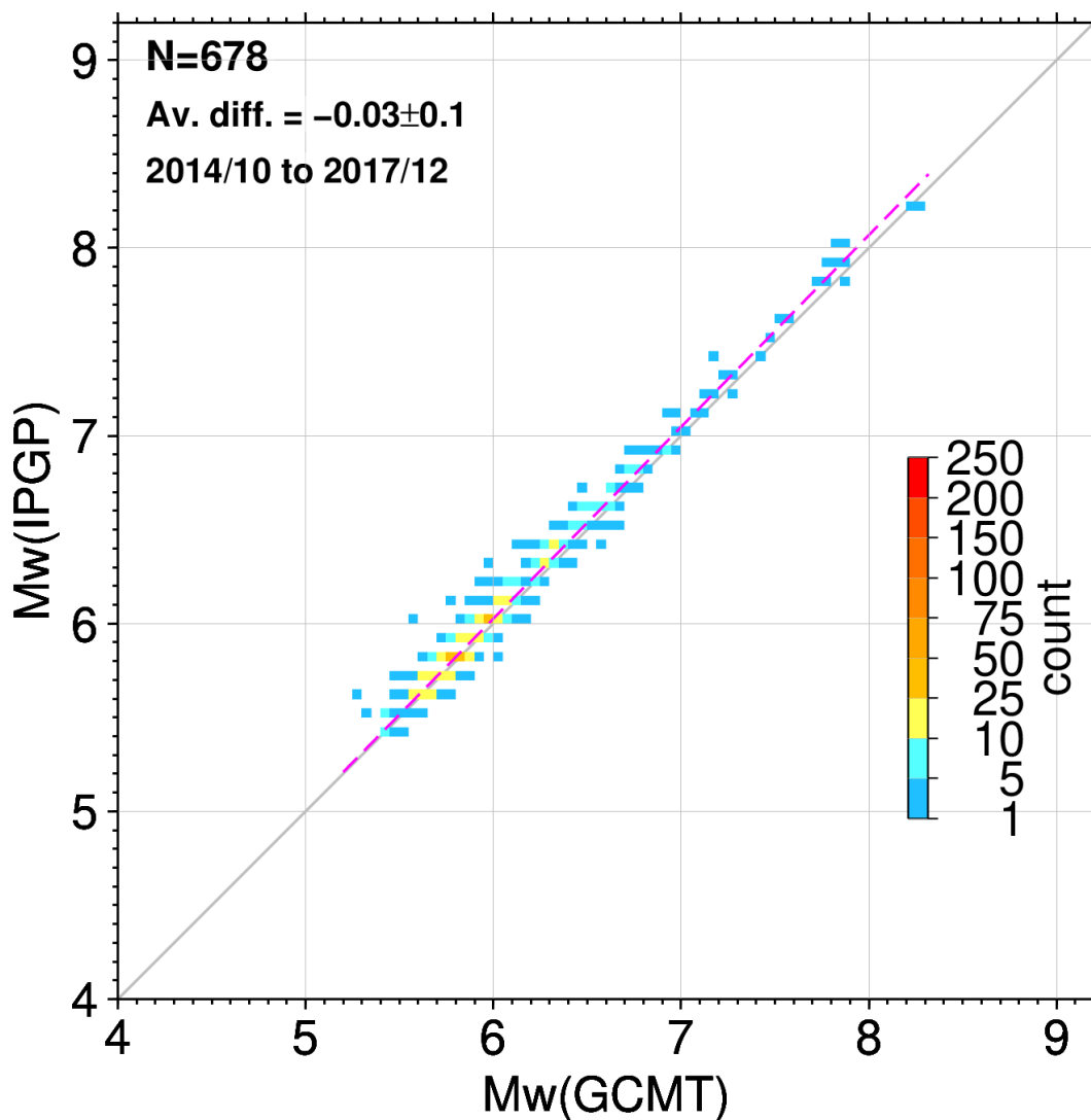
Figure A17. As for Fig. 8 but for GCMT and IPGP.
