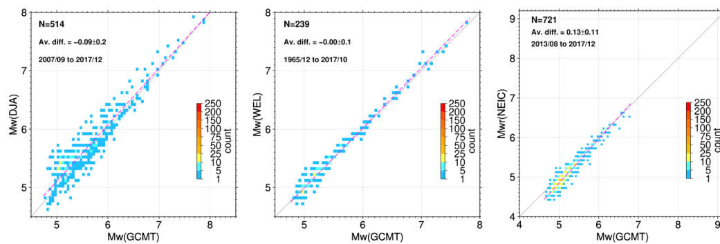
Figure A18. As for Fig. 8 but for GCMT and DJA (left), GCMT and WEL (middle), GCMT and M_w NEIC (right).
