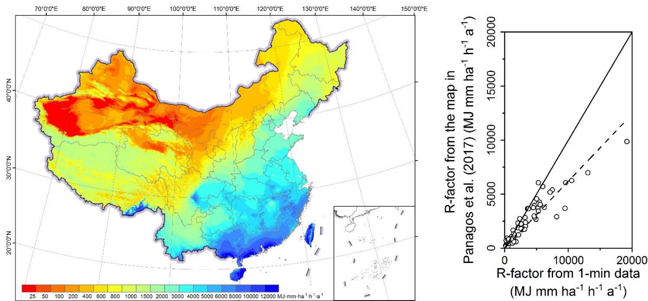
385 Figure 12: R-factor map for China extracted from Panagos et al. (2017) and the evaluation of the map based on 62 stations with 1-min data.
