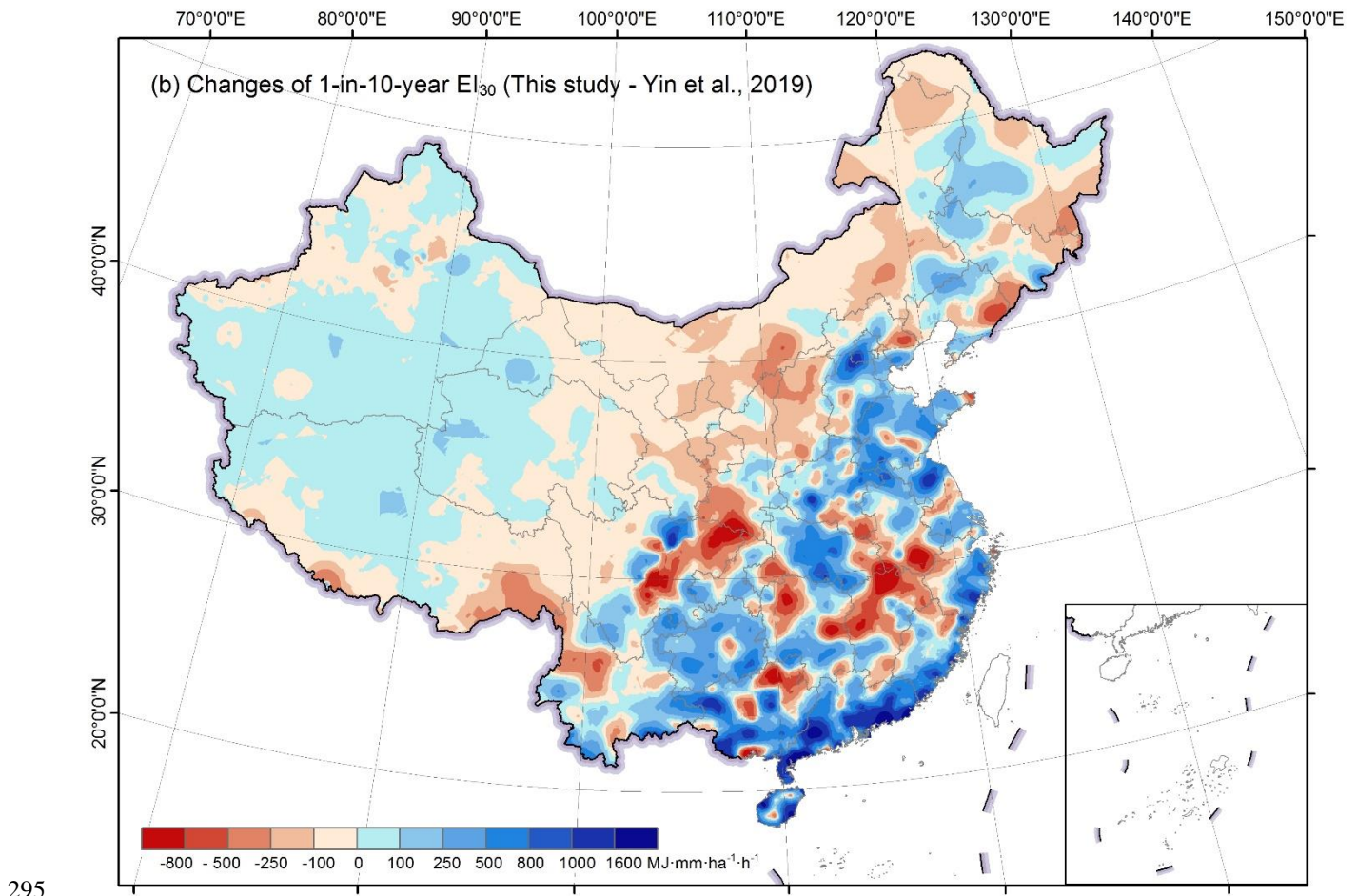
Figure 9: Differences of the R-factor(a) and the 1-in-10-year EI_{30} (b) comparing with the previous study
