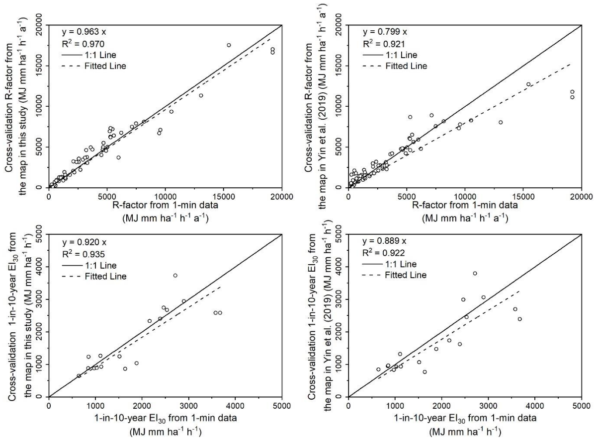
265 Figure 4: Comparison of the R-factors and 1-in-10-year EI_{30} of the cross-validation values at the station of the maps and the values from 1-min data. The graphs on the left were the evaluation of the maps generated in this study, and those on the right were the evaluation of the maps generated by Yin et al. (2019)
