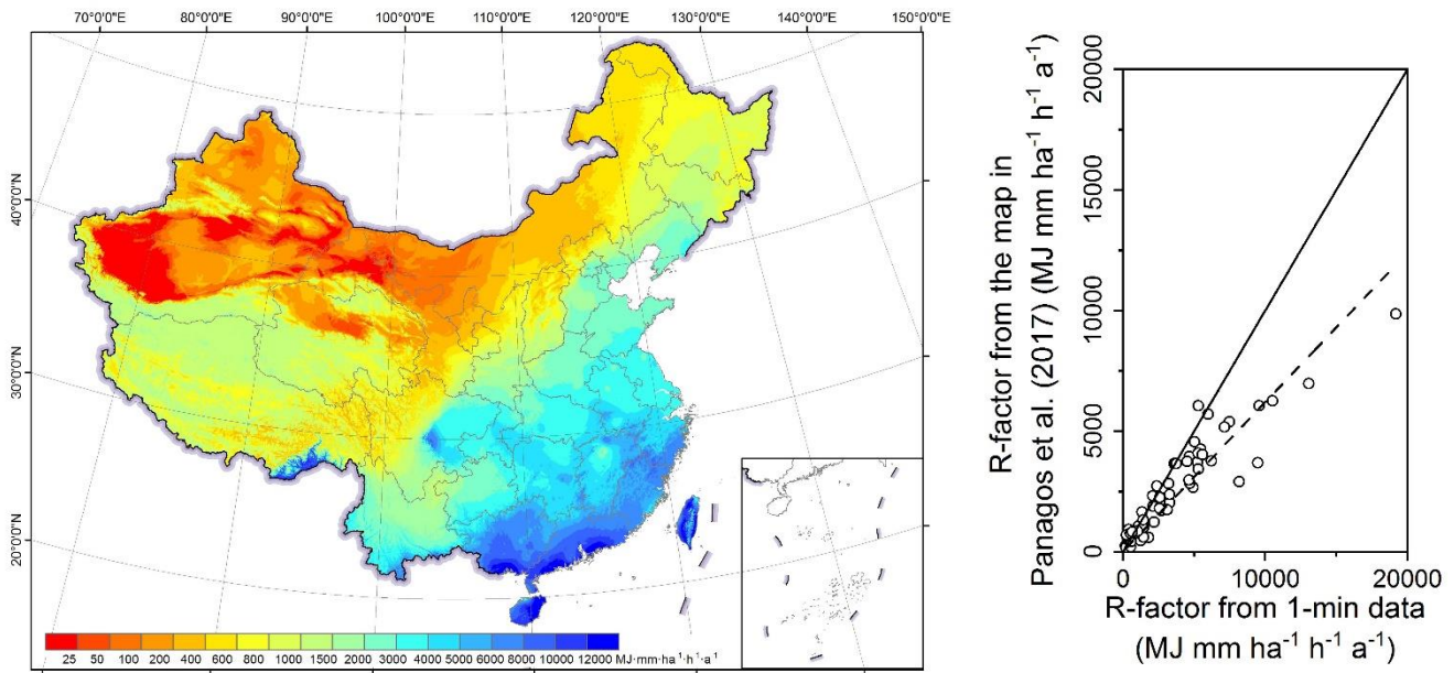
390 Figure 12: R-factor map for China extracted from Panagos et al. (2017) and the evaluation of the map based on 62 stations with 1-min data.
