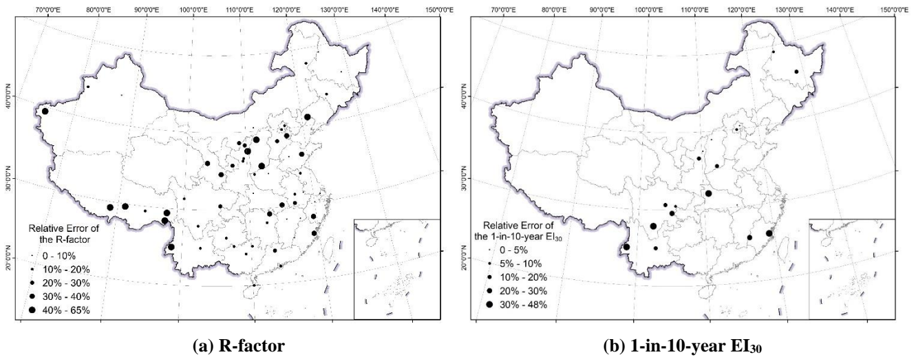
275 Figure 66: Spatial distribution of the absolute relative errors in the map of R-factor for 62 stations (a) and in the map of 1-in-10-year EI 30 for 18 stations (b) with 1-min observation data.
