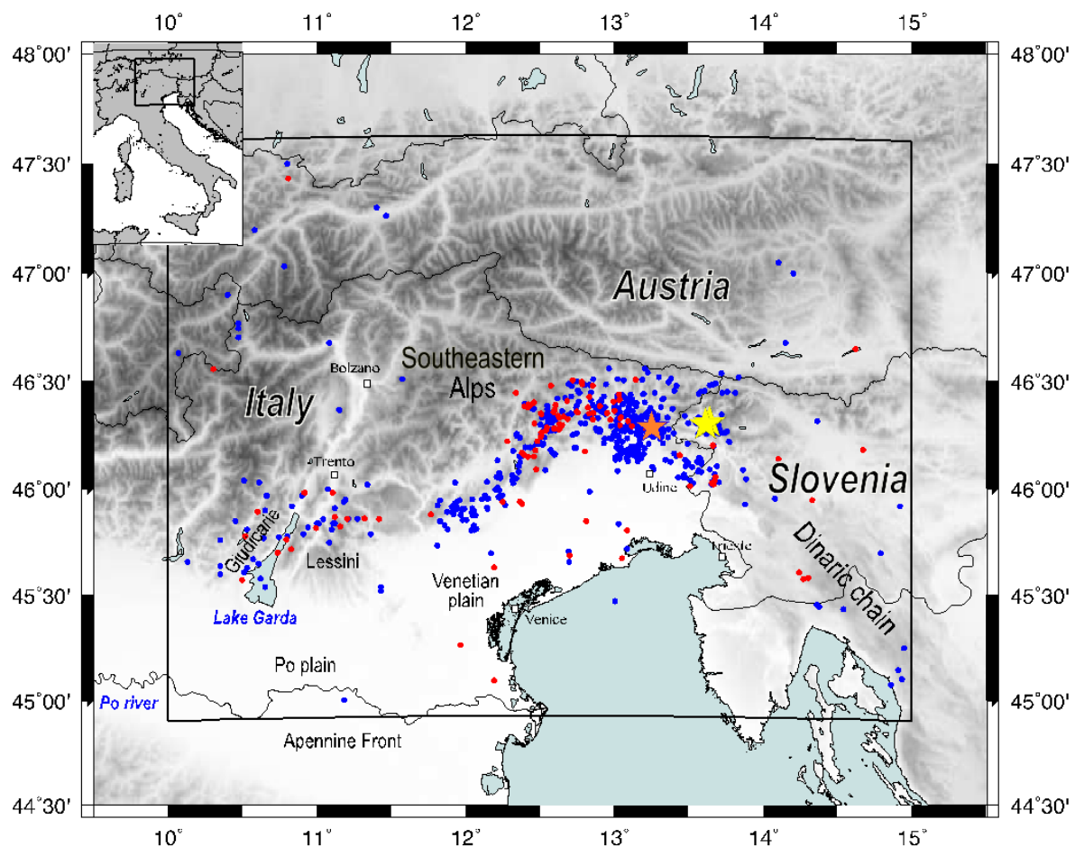
Figure 1: Map of the epicentres of the focal mechanisms reported in the catalogue (Saraò et al., 2020,2021) presented in this paper. The epicentres of the focal mechanisms retrieved from the literature are indicated by the blue dots, and the newly computed FPSs are indicated by the red dots. The 1976 Friuli earthquake (orange star) and the 1998 and 2004 Bovec earthquakes (yellow stars) are also shown. The map was generated by GMT software (Wessel et al., 2019).
