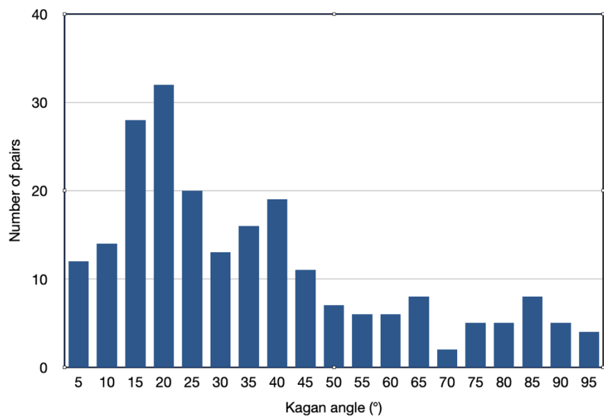
Figure 7 - Kagan angle between the preferred solution and the alternative multiple focal mechanism solutions FPS reported in our catalogue.
