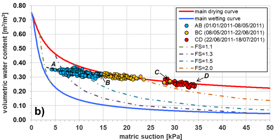
315 Figure 10: Volumetric water content and matric suction recorded from January to July, 2011 at depths z = 0.60 m (a) and z = 1.00 m (b) and iso-Safety Factor curves. The main drying curve at z = 0.60 m is obtained fitting with the Eq. (1) all the experimental points monitored from 08/05/2011 to 18/07/2011 (the fitted parameters are shown by Table 4). The main drying curve at z = 1.00 m is obtained fitting with the Eq. (1) all the experimental points monitored from 07/06/2011 to 18/07/2011 (the fitted parameters are shown by Table 5). The main wetting curves at both depths coincide with that derived by the infiltration tests (Damiano and Olivares, 2010) shown in Figure 6. The safety factor, FS, is calculated by Eq. (2), provided by the simplified infinite slope model, assuming a homogeneous deposit with slope angle \alpha = 40^\circ , unit weight \gamma = 14 kN/m 3 , cohesion c' = 0 , friction angle \varphi' = 38^\circ , \theta_s = 0.75 m 3 /m 3 , \theta_r = 0 . 320
