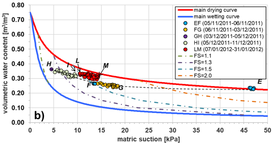
360 Figure 12: Volumetric water content and matric suction, monitored from November, 2011 to January, 2012 at depths z = 0.60 m (a) and z = 1.00 m (b), and iso-Safety Factor curves. The main drying curve at z = 0.60 m is obtained fitting with the Eq. (1) all the experimental points monitored from 08/05/2011 to 18/07/2011 (the fitted parameters are shown by Table 4). The main drying curve at z = 1.00 m is obtained fitting with the Eq. (1) all the experimental points monitored from 07/06/2011 to 18/07/2011 (the fitted parameters are shown by Table 5). The main wetting curves at both depths coincide with that derived by the infiltration tests (Damiano and Olivares, 2010) shown in Figure 6. The safety factor, FS, has been calculated by Eq. (2), provided by the simplified infinite slope model, assuming a homogeneous deposit with slope angle \alpha = 40^\circ , unit weight \gamma = 14 \text{ kN/m}^3 , cohesion c' = 0 , friction angle \phi' = 38^\circ , \theta_s = 0.75 \text{ m}^3/\text{m}^3 , \theta_r = 0 . 365
