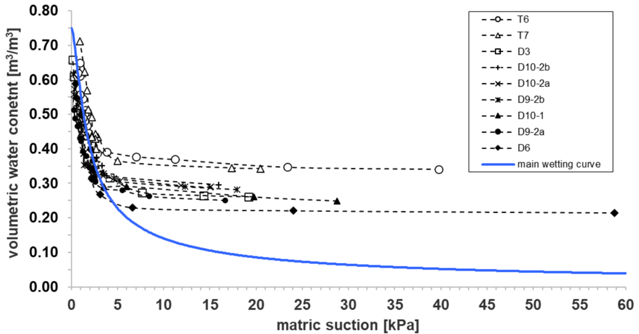
160 Figure 6: Coupled values of matric suction and volumetric water content measured during infiltration tests (Damiano and Olivares, 2010). The tests acronyms shown in the legend are those reported in the repository dataset (Comegna et al., 2020). The main wetting curve is obtained fitting all the experimental points featured by matric suction values lower than 4 kPa with the van Genuchten Eq. (1). The fitted van Genuchten parameters are shown by Table 2.
