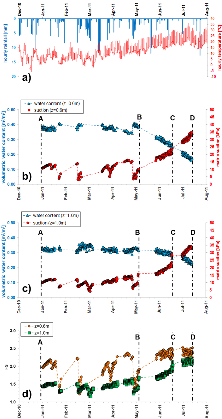
310 Figure 9: Hourly weather data (a), matric suction and volumetric water content monitored from January to July, 2011 at depth z = 0.60 m (b) and z = 1.00 (c), factor of safety, FS (d), calculated by Eq. (2), provided by the simplified infinite slope model, assuming a homogeneous deposit with slope angle \alpha = 40^\circ , unit weight \gamma = 14 kN/m 3 , cohesion c' = 0 , friction angle \varphi' = 38^\circ , \theta_s = 0.75 m 3 /m 3 , \theta_r = 0 .
