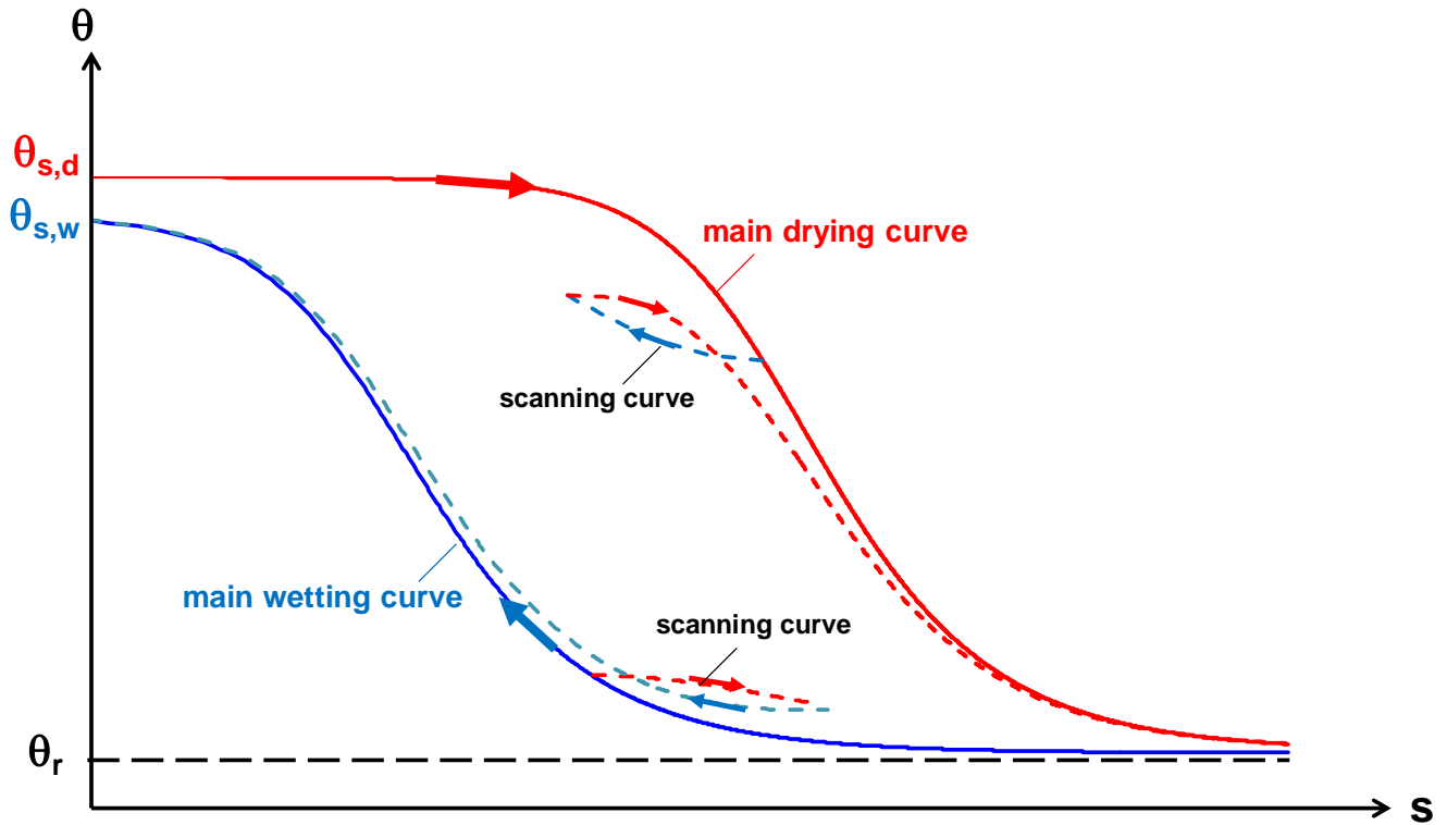
Figure 1: Typical hydraulic response of a soil sample subjected to drying and wetting cycles. Along the main drying curve , the volumetric water content, \theta , continuously decreases with the matric suction, s , from the initial saturated value, \theta_{s,d} , until the minimum residual value, \theta_r , is reached. Along the main wetting curve , \theta continuously increases from the initial residual value, \theta_r , until the final maximum value, \theta_{s,w} , is reached at s = 0 . If the continuous main drying (wetting) stage is interrupted by a reverse wetting (drying) process, a different scanning curve , located under (over) the main path, is travelled.
