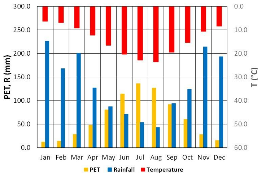
115 Figure 4: Mean monthly values of rainfall depth, R, temperature, T, and potential evapotranspiration, PET. R is calculated with the 2001-2017 data from the rain gauge installed in Cervinara by the meteorological alert network managed by the “Functional Centre for forecast, prevention and monitoring of risks and alerting for civil protection” of Campania Civil Protection Agency. T is 120 calculated with the data monitored from 1979 to 1998 by the meteorological station of Montesarchio, managed by the National Hydrological Service. PET is estimated with the Thornthwaite expression (1946).
