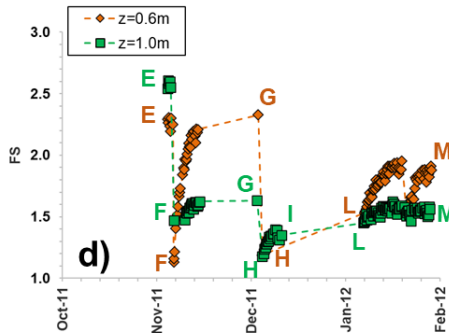
Figure 11: Monitored hourly weather data (a), matric suction and volumetric water content from November, 2011 to January, 2012 at the depth z = 0.60 m (b) and z = 1.00 (c), factor of safety, FS (d), calculated by Eq. (2), provided by the simplified infinite slope model, assuming a homogeneous deposit with slope angle \alpha = 40^\circ , unit weight \gamma = 14 \text{ kN/m}^3 , cohesion c' = 0 , friction angle \phi' = 38^\circ , \theta_s = 0.75 \text{ m}^3/\text{m}^3 , \theta = 0 .
