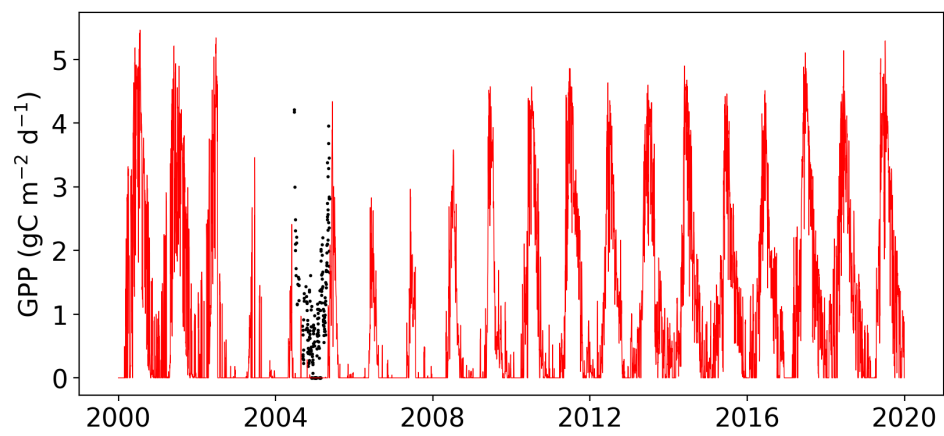
Fig. 1. Figure R1. Comparison between AmeriFlux (black dots) and SLOPE (red curves) daily GPP at the US-Me1 site, which shows the lowest R2.
