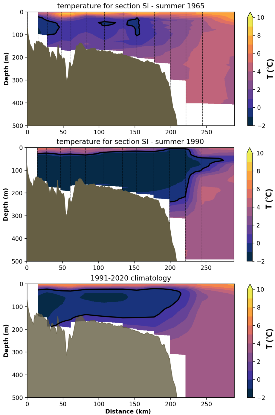
Figure 9. Summer temperature along hydrographic section Seal Island (SI) during 1965 (top), 1990 (center) and the 1991-2020 average (bottom). The vertical axis is limited to the top 500 m and the horizontal axis is the distance (in km) from the coast. The CIL ( T < 0^{\circ}\text{C} ) is highlighted with a thick black contour. Stations location are indicated with thin dashed lines.
