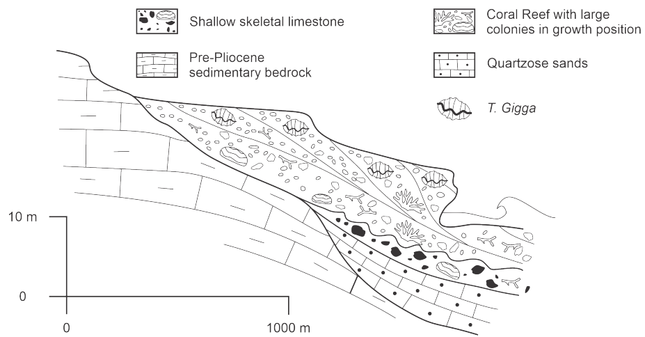
Figure 4. Litholog of raised emerged reef coast of Kenya (Modified after Accordi et al. (2010)).
