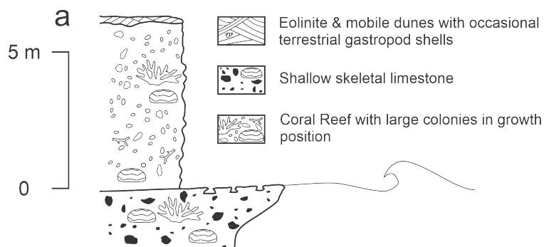
Figure 5. (a) Litholog of raised-merged reef near Dar-es-Salaam (Modified after Battistini (1966)). (b) Ras Mwanamkuru just south of Ras Kankadya. Exposed Pleistocene reef sitting atop poorly consolidated skeletal limestone. Approximately 10 - 15 m tall. Photo by D.Oppo.
