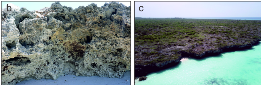
Figure 6. (a) Litholog of Marine Terrace II (Modified after Korotky et al. (1992)). (b) Lower part of the Pleistocene reef complex at Aldabra Island. (c) Aerial view of the Pleistocene reef at Assumption Island. Photos by A. Rovere.
