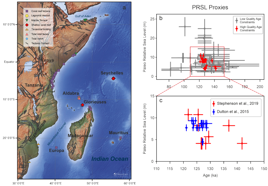
Figure 2. Paleo Relative Sea Level Indicators of the East Africa and Western Indian Ocean Region. (a) Overview map showing the distribution of PRSL proxies and their respective indicator types. (b) Overview of age and elevation distribution. Proxies with age constraints with a quality rating lower than 4 within WALIS are colored grey and those proxies with a quality rating of 4 or greater are colored red. The elevations refer to paleo relative sea level. “Relative 22 ” means that they are still uncorrected for any post-depositional vertical movement, such as, for example, tectonics or GIA. (c) The high quality age constraints are from two areas, Northern Madagascar (Stephenson et al., 2019) and the Granite-granitic Seychelles (Dutton et al., 2015).
