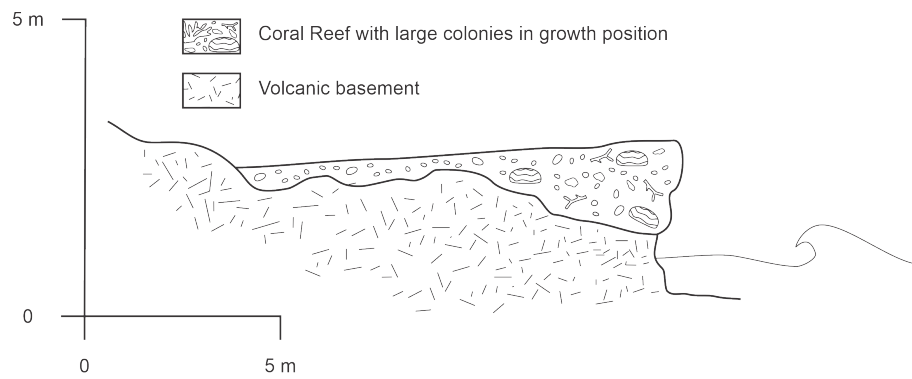
Figure 7. Raised reef platform of Île Plate (Modified after Montaggioni (1982)).
