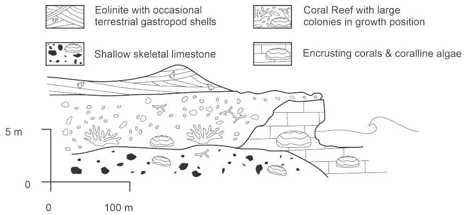
Figure 3. Raised reef and aeolinites of southern Somalia (Modified after Carbone and Accordi (2000)).
