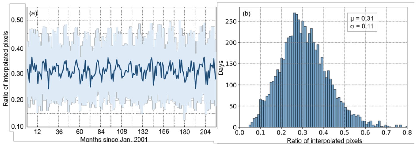
650 Figure A2. Ratio of interpolated pixels of land surface temperature (MOD11) data: (a) time series of interpolated pixels per month over 2001–2018 and (b) histogram of ratio of interpolated pixels.
