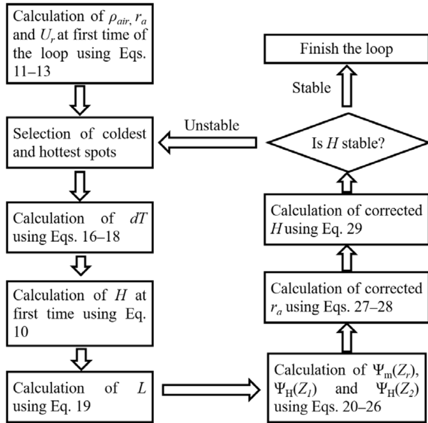
645 Figure A1. A flowchart of the calculation of sensible heat flux using Monin–Obkhov Similarity Theory (MOST).
