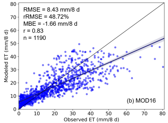
Figure 9. The results of the overall validation. (a) SEBAL ET validation at the 8-day scale; (b) MOD16 ET validation at the 8-day scale.
