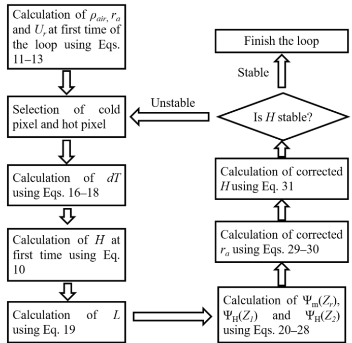
Figure A1. A flowchart of the calculation of sensible heat flux using Monin–Obkhov Similarity Theory (MOST).
