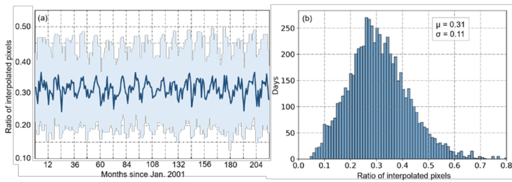
Figure A2. Ratio of interpolated pixels of land surface temperature (MOD11) data: (a) time series of interpolated pixels per month
