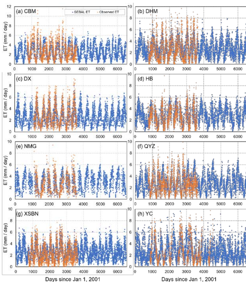
245 Figure 4. The SEBAL ET and flux tower observed ET variation in time series. (a) CBM; (b) DHM; (c) DX; (d) HB; (e) NMG; (f) QYZ; (g) XSBN and (h) YC.
