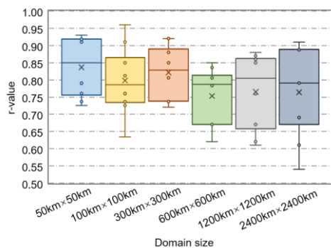
485 Figure 12. The performance of different domain sizes used in SEBAL ET estimates.
