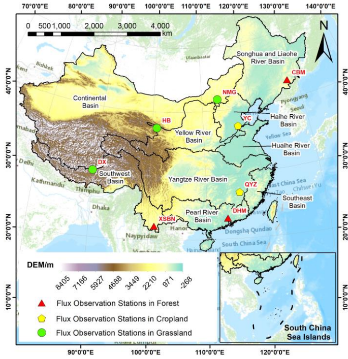
110 Figure 1. The location of the study area. Note: CBM: Changbai mountain; DHM: Dinghu mountain; DX: Dangxiong; HB: Haibei; NMG: Neimenggu; QYZ: Qianyanzhou; XSBN: Xishuangbanna; YC: Yucheng. (Note: the Chinese boundary was obtained from Institute of Geographic Science and Natural Resources Research, Chinese Academy of Sciences ( http://www.resdc.cn/ ))
