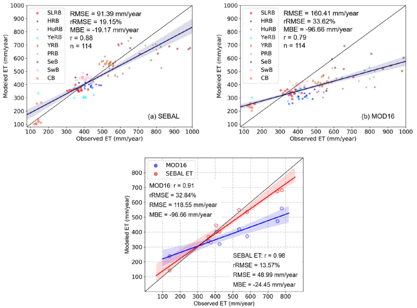
Figure 10. The results of validation at the basin-scale.
