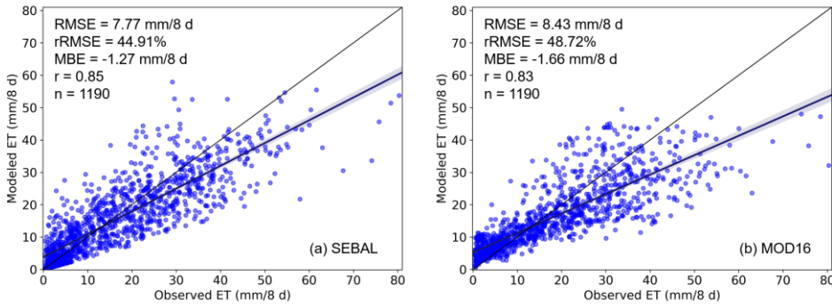
425 Figure 9. The results of the overall validation. (a) SEBAL ET validation at the 8-day scale; (b) MOD16 ET validation at the 8-day scale.
