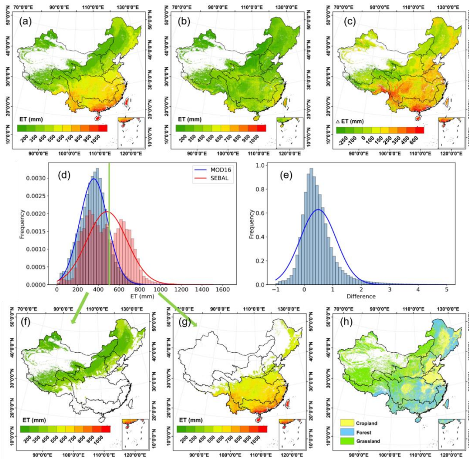
Figure 11. A comparison between the SEBAL and MOD16 models. (a) Distribution of annual average ET_{SEBAL} ; (b) Distribution of annual average ET_{MOD} ; (c) Distribution of the difference between SEBAL and MOD16 ( ET_{SEBAL} - ET_{MOD} ); (d) Histogram of annual average ET_{SEBAL} and ET_{MOD} ; (e) Histogram of the relative difference between SEBAL and MOD16 ( (ET_{SEBAL} - ET_{MOD})/ET_{MOD} ); (f) Map of ET_{SEBAL} over 500 mm; (g) Map of ET_{SEBAL} below 500 mm; (h) Land cover in China.
