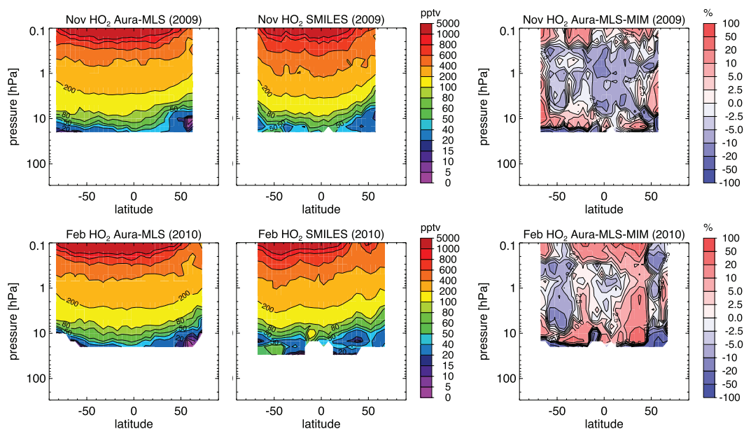
Figure 14. zonal monthly mean \text{HO}_2 cross sections for Aura-MLS and SMILES daytime (LT) data (left two columns) and Aura-MLS relative differences from the MIM (right column) are shown for November 2009 (upper row) and February 2010 (lower row), respectively. Note, the SMILES relative differences from the MIM would look exactly opposite of these figures and thus are not shown.
