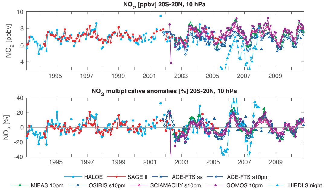
Figure 13. Time series of tropical \text{NO}_2 mean values (upper panels) and deseasonalized anomalies (lower panels) between 20°S-20°N at 10 hPa for 1993-2010. Data sets correspond to local sunset or to 10 pm LSTs as described in the text. The s10pm denotes zonal monthly mean fields scaled to 10 pm, the ss zonal monthly mean fields from sunset measurements.
