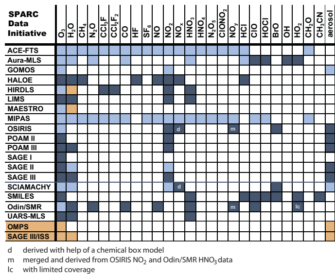
Figure 2. Coloured boxes indicate SPARC Data Initiative zonal monthly mean timeseries of atmospheric constituents, listed by instruments and available from Zenodo (doi:10.5281/zenodo.4265393). Dark blue are timeseries originally submitted and evaluated in SPARC (2017), light blue updated timeseries based on new data versions, and orange newly added instruments and/or timeseries.
