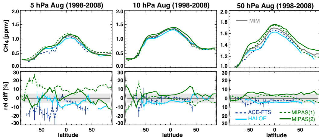
Figure 8. Meridional profiles of zonal monthly mean \text{CH}_4 at 5, 10, and 50 hPa and averaged over 1998-2008 are shown for the different instruments and the MIM (upper panels). Differences between the individual instruments and the MIM are shown in the lower panels. The grey shading indicates where the relative differences are smaller than \pm 5\% (thus where the datasets show very good to excellent agreement). Error bars indicate the uncertainty in the relative differences based on the SEM of each instrument.
