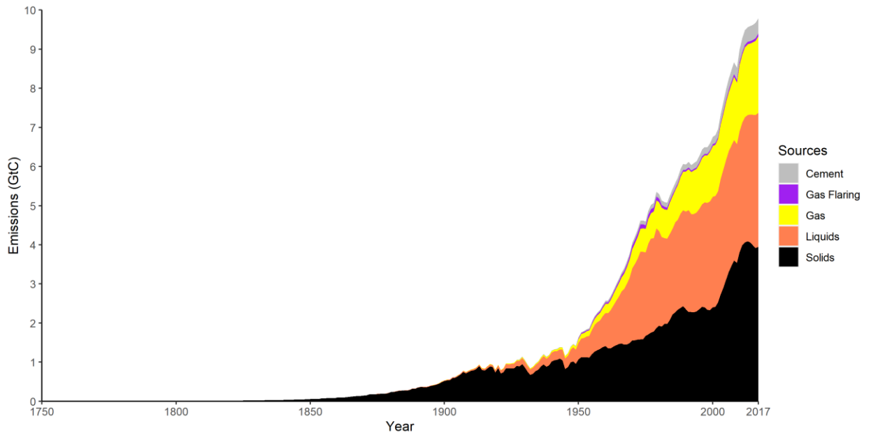
420 Figure 2. Total global CO 2 emissions from fossil fuel combustion and cement manufacture
