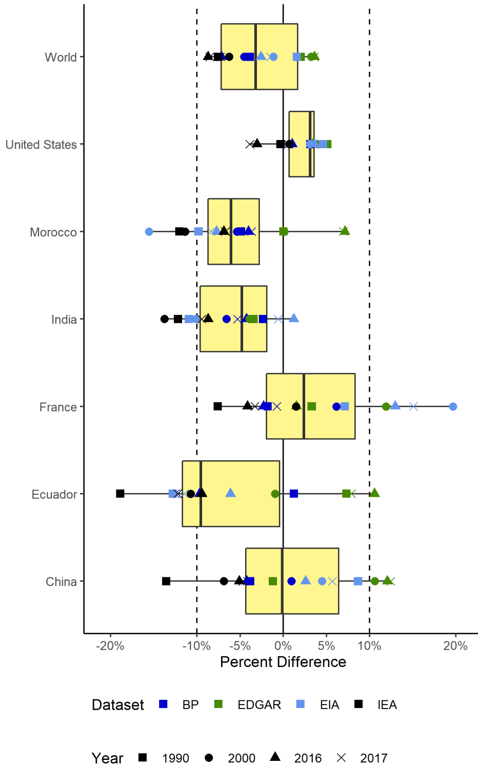
Figure 3. Comparison of four other global emissions datasets with CDIAC-FF for 1990, 2000, 2016, and 2017. Specific emissions datasets are cited in section 2.1. The 0% centerline represents exact agreement with the CDIAC-FF value. Six countries and the global totals were selected to illustrate the variability between datasets and countries. Shapes represent
