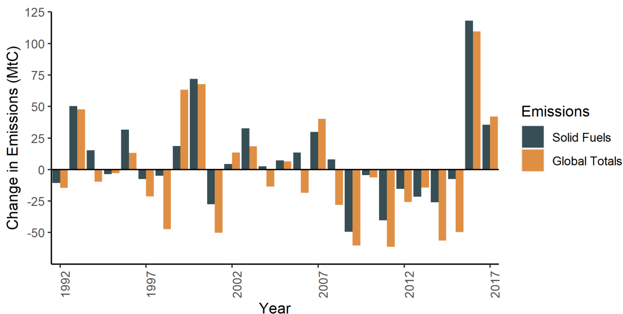
275 Figure 1. The change in estimated global total CO 2 emissions by including changes in stocks as opposed to just using production data, in million tons of carbon (MtC). In 2016, the change in global total emissions (orange) corresponds to a 1.10 % underestimation of emissions if drawdown of stocks is not included in the calculation of global total emissions.
