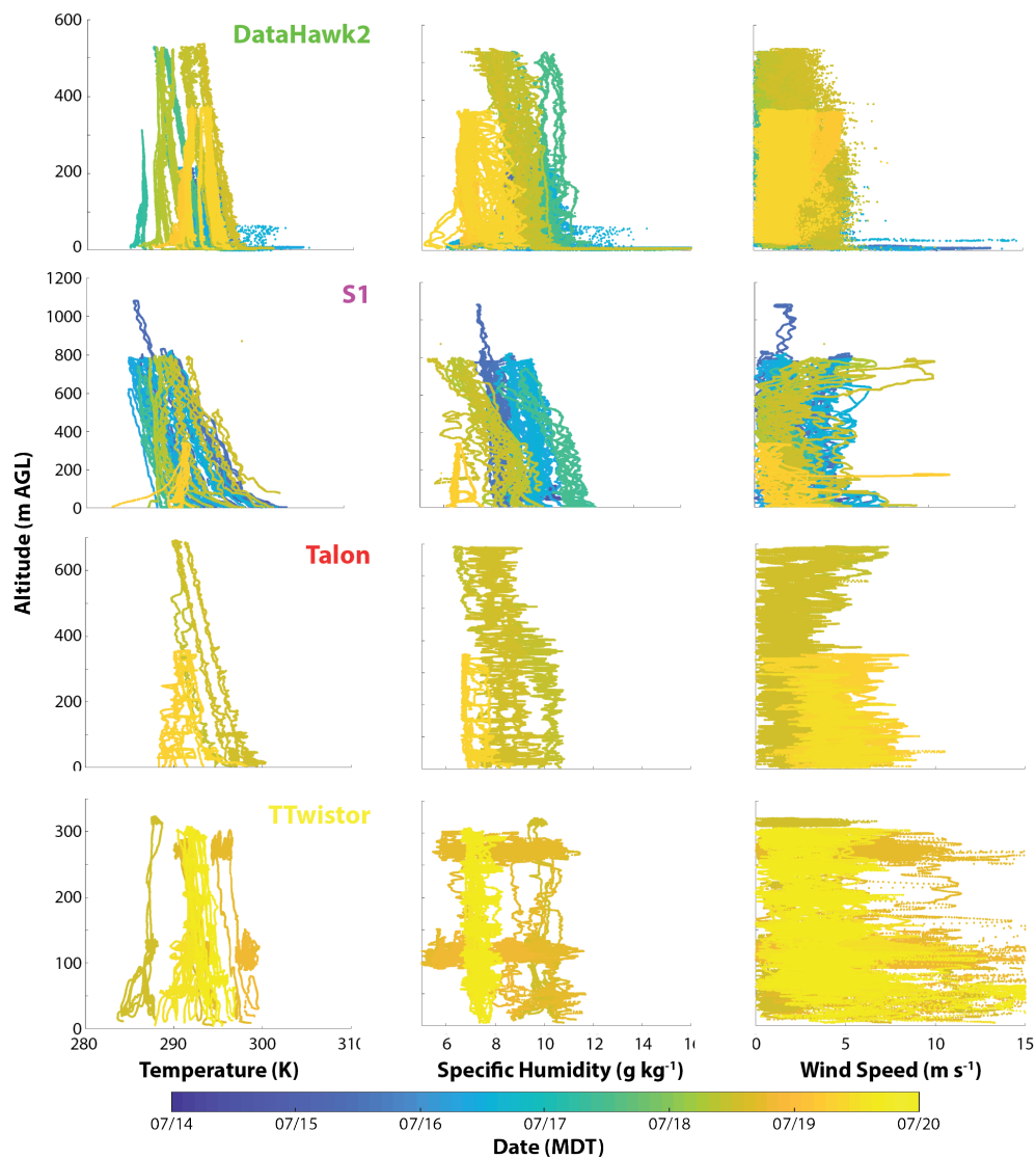
Figure 7: Profiles of (left to right) temperature, specific humidity and wind speed from the DataHawk2, S1, Talon and TTwistor (top to bottom). Colors indicate the date of flight.
