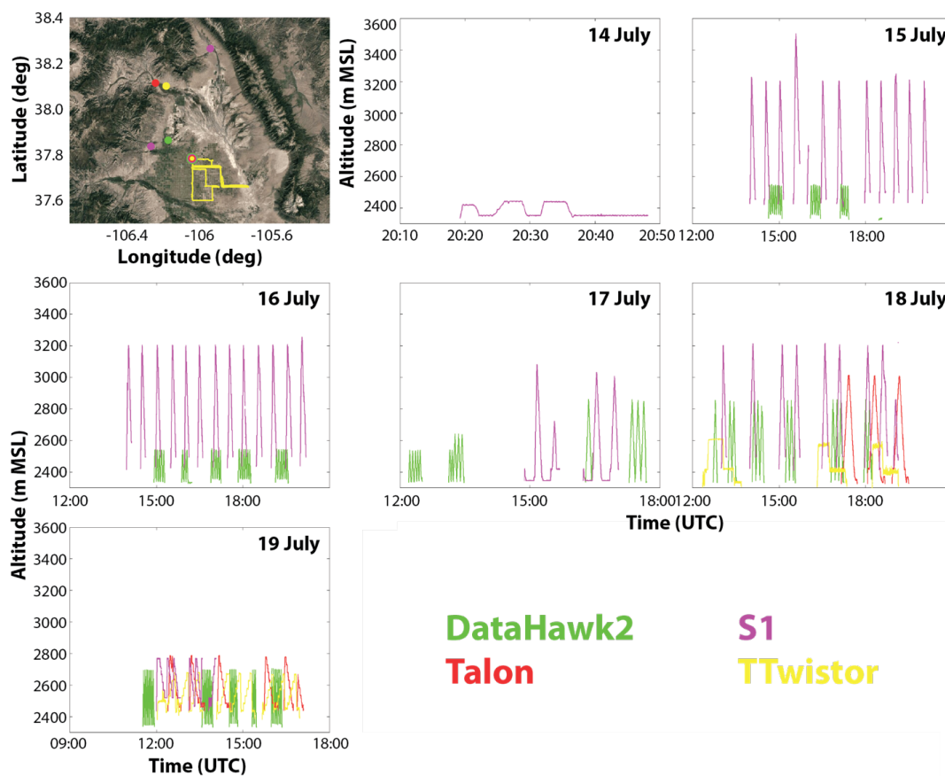
Figure 2: The flight locations for each aircraft (left) and altitudes covered by the different aircraft broken down by day (right). Map background is from © Google Maps, downloaded through their API.
