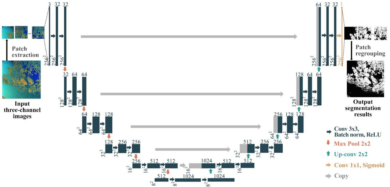
265 Figure 7. The overall architecture of the proposed sea ice segmentation model for the S1 EW data based on the U-Net deep learning algorithm.
