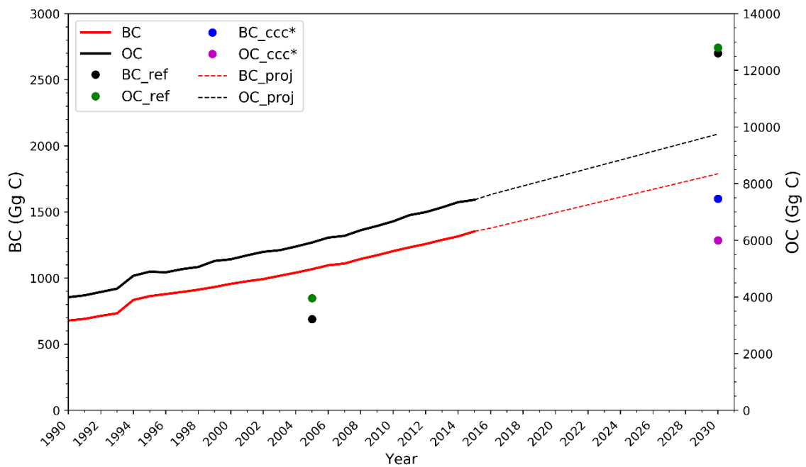
Figure S1: Comparison of OC and BC emissions between DACCIWA inventory (this work in solid line and its projection in dash line) and Lioussé et al. (2014) inventory (in dot).
