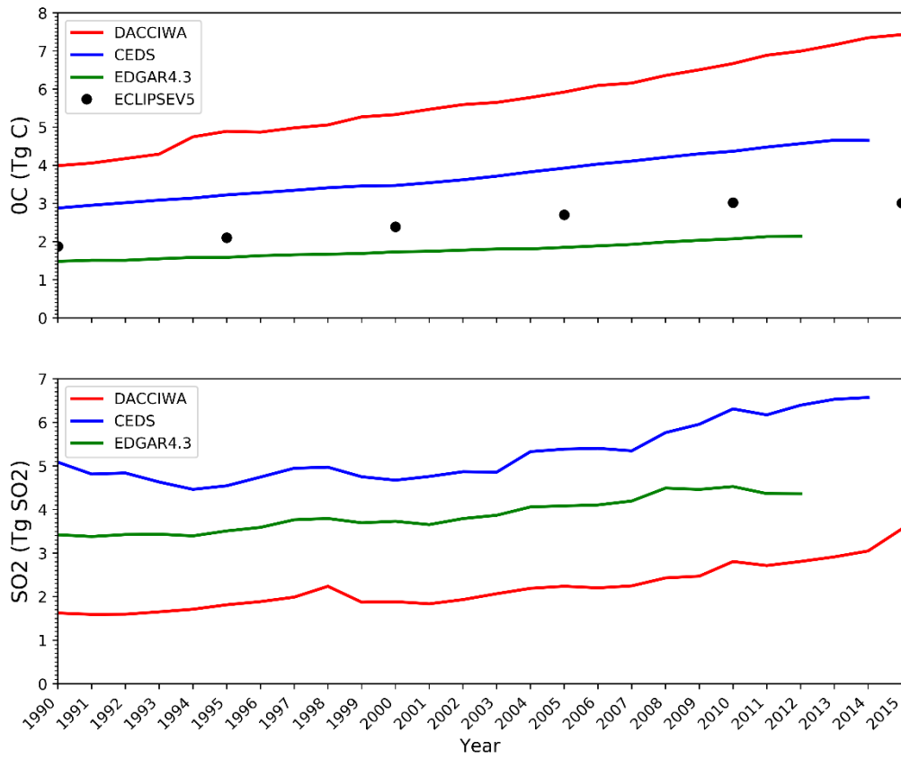
Figure S2: Comparison of OC (top) and SO 2 (bottom) between DACCIWA inventory (this work) and global inventories (CEDS, EDGAR and ECLIPSE inventories).
