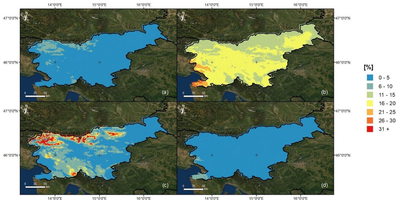
295 Figure 11: Uncertainty of a) TXx - absolute daily maximum temperature, b) TNn - absolute daily minimum temperature, c) SU - number of summer days and d) FD - number of frost days (Esri, 2020; GISCO, 2020).
