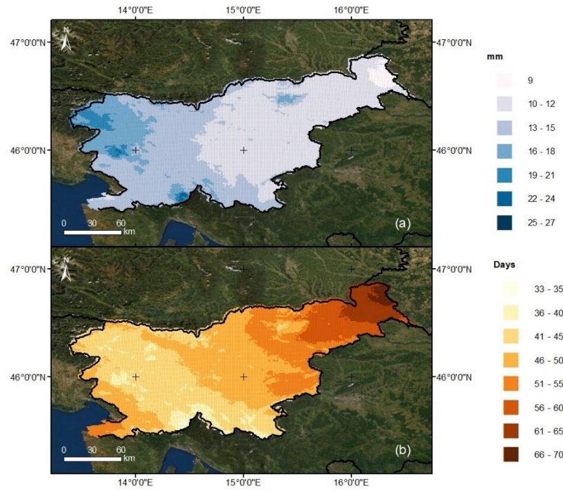
285 Figure 8: Daily precipitation indices: (a) SDII - daily precipitation intensity, (b) CDD - maximum number of consecutive dry days (Esri, 2020; GISCO, 2020).
