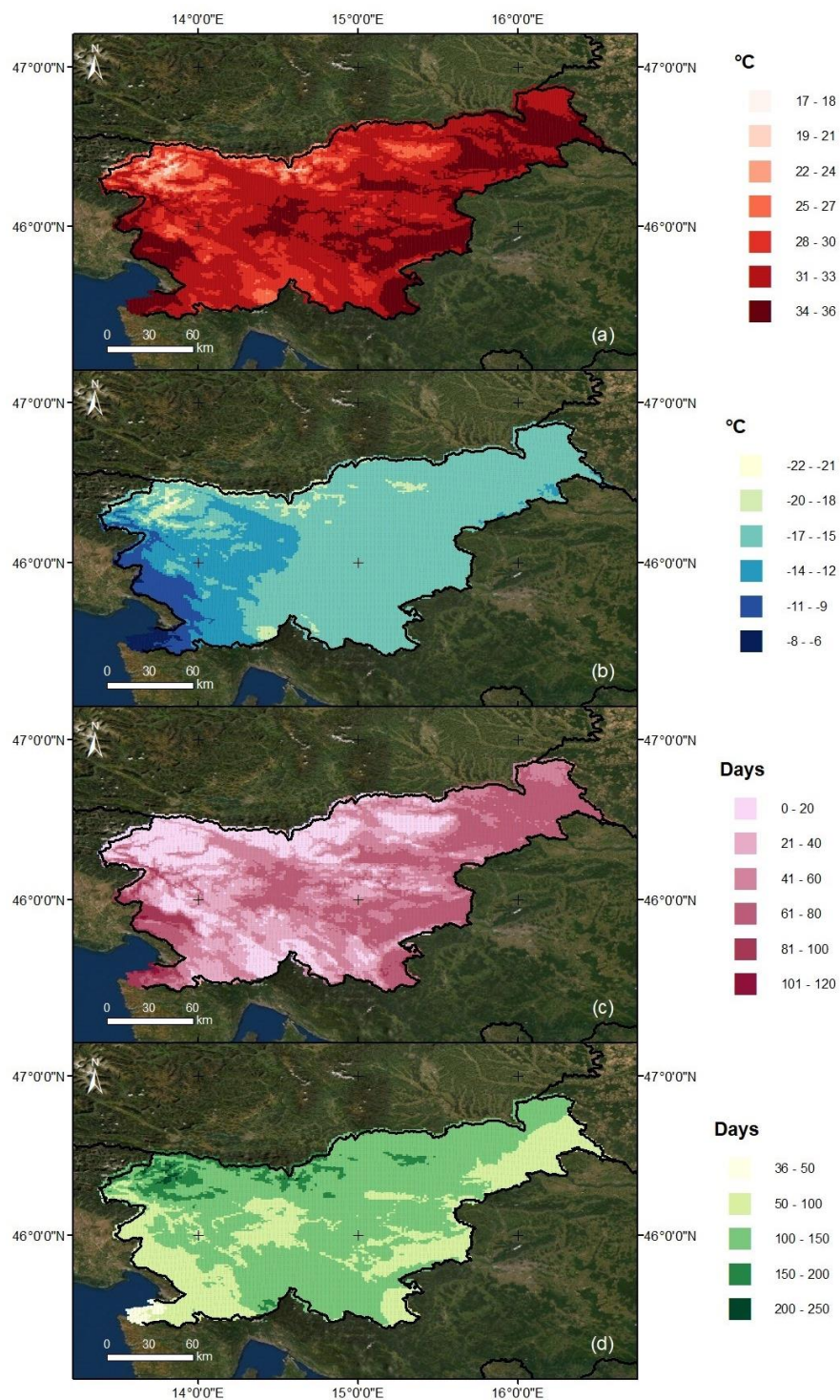
290 Figure 10: Mean annual (1950-2018) values for (a) TXx - absolute daily maximum temperature, (b) TNn – absolute daily minimum temperature, (c) SU - number of summer days, (d) FD - number of frost days (Esri, 2020; GISCO, 2020).
