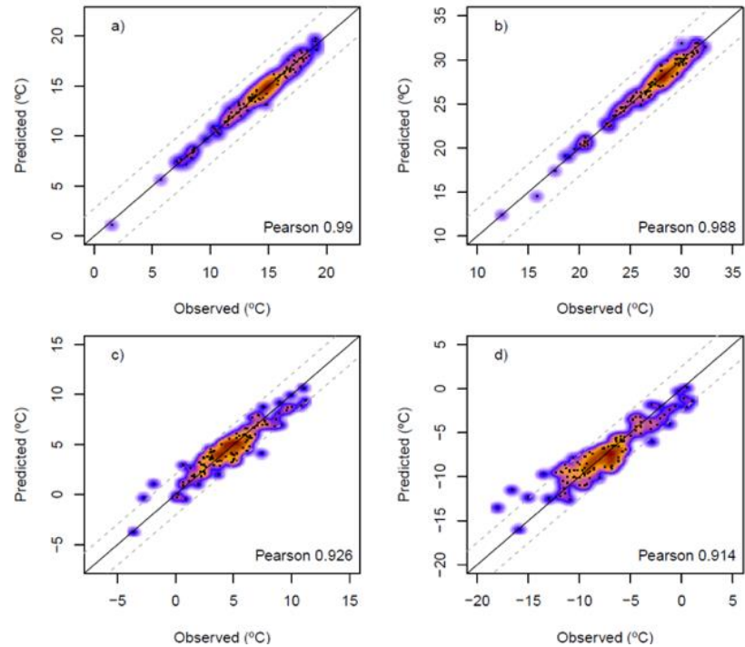
230 Figure 6: Comparison between measurements and estimates, by stations, of the mean maximum temperatures (a) and their 95th percentiles (b), and comparison of the mean minimum temperatures (c) and their 5th percentiles (d). Dashed lines represent \pm 1 standard deviation of the data.
