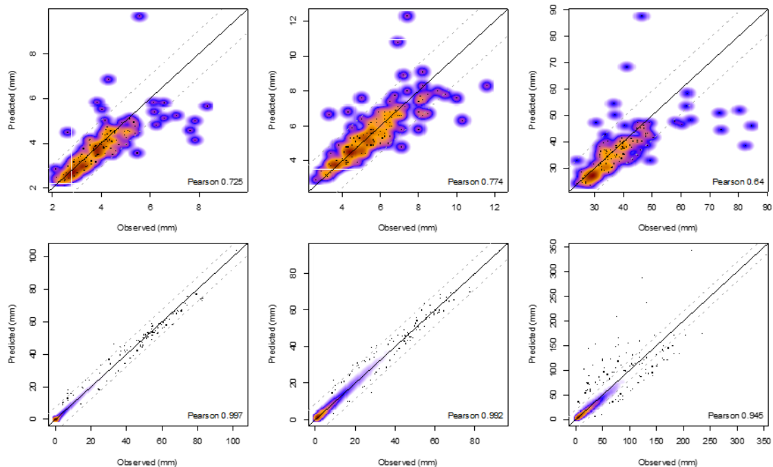
Figure 4: Comparison between measurements and estimates by stations (upper row) and by days (lower row). Left column: comparison of mean precipitation; central column: comparison of median precipitation in wet days; right column: comparison of 95th percentiles in wet days. Dashed lines represent \pm 1 standard deviation of the data.
