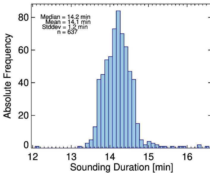
325 Figure 8: Measurement duration for all dropsonde with normal parachute behavior reaching the surface.
