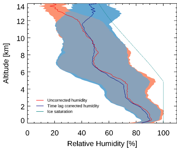
310 Figure 4: Mean relative humidity profile for all OTREC soundings. The average of the uncorrected relative humidity is shown in red, the average of the time lag corrected relative humidity is shown in blue. The standard deviation for each is shown as shaded areas. Saturation over ice is shown as solid green line.
