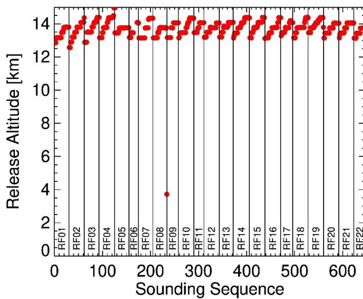
315 Figure 5: Time series of the release altitudes during OTREC. Sonde were typically launched above 12.1 km. Vertical lines separate the research flights, which are indicated near the bottom. The last sounding of RF08 was launched at low altitude due to operational reasons.
