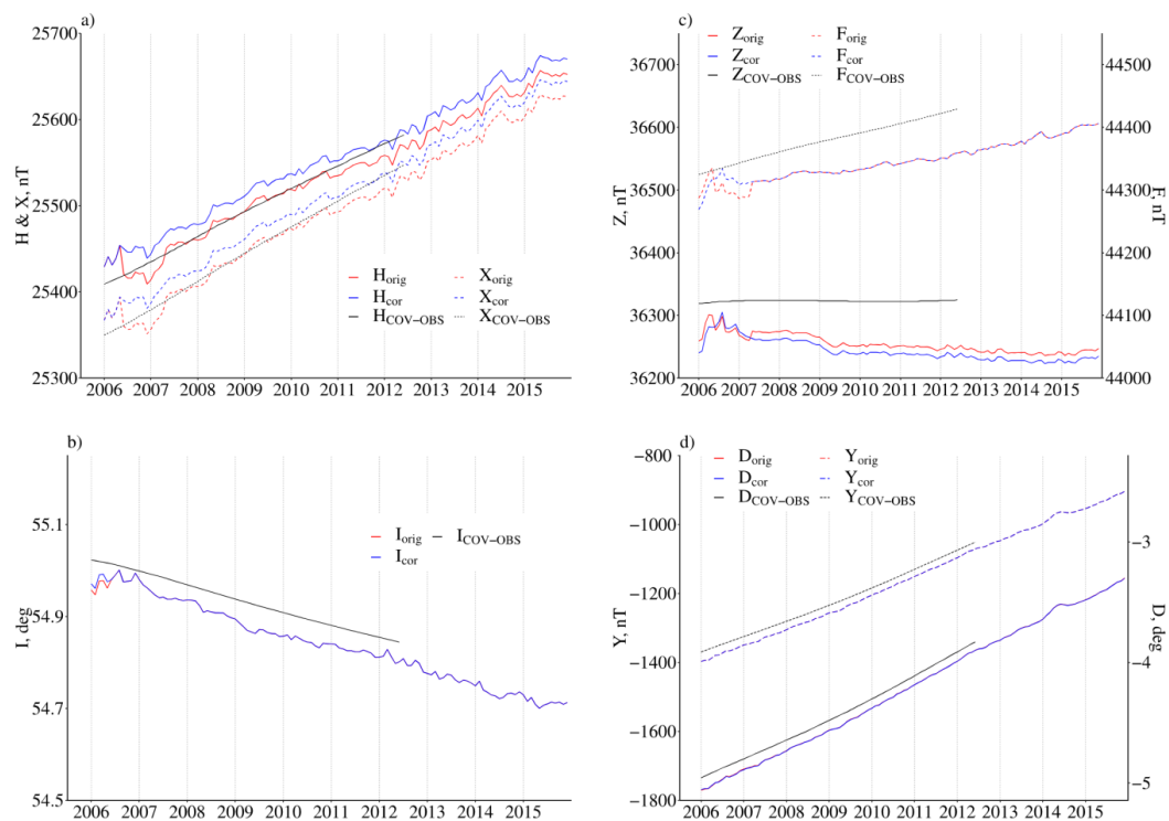
Figure 8. Same as Figure 1 but from 2006 to 2015.
