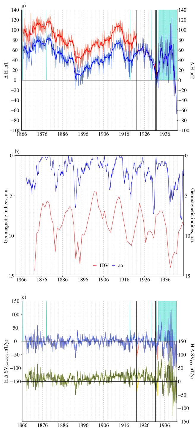
540 Figure 2: (a) Original (red) and corrected (blue) COI \Delta H series for the C-AdB period of measurements: 1866-1941. Thin lines are data and thick lines are moving average with 12-month span window. (b) Variations of the geomagnetic indices aa (monthly data, blue) and IDV (annual data, red). Please note reversed Y axis. (c) Original (red) and corrected (blue) \Delta SV_{\text{COV-OBS}} series for H; original (yellow) and corrected (green) \Delta SV_{\text{EO}} series for H. Cyan vertical lines/rectangles mark possible HBs which are not corrected (see details in the text), black vertical lines mark dates of the corrected HBs.
