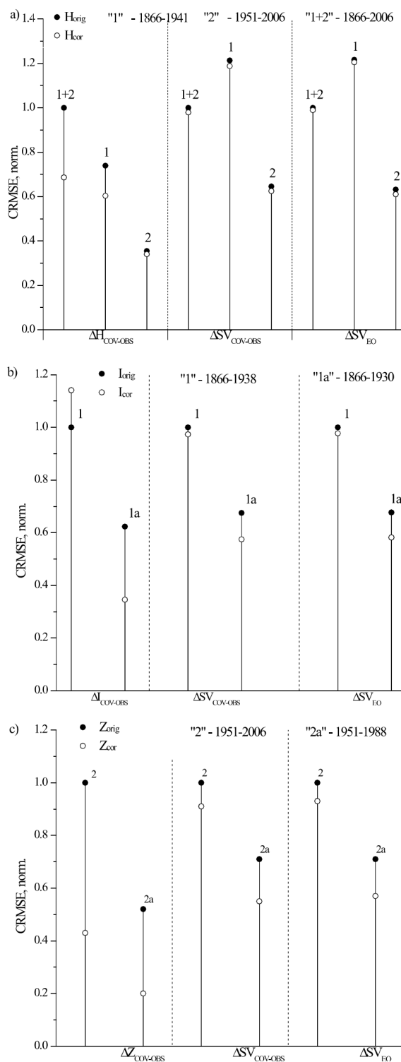
555 Figure 7. CRMSE of the original (black dots) and corrected (white filled circles) COI series estimated for different time intervals: a - COI H, b - COI I, c - COI Z. CRMSE values are normalized by the standard deviations of the original series.
