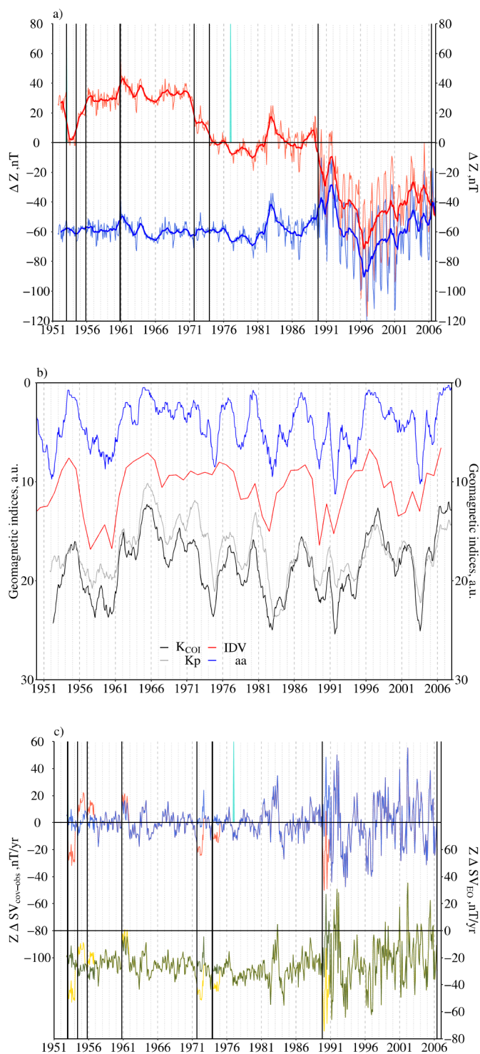
550 Figure 5: Same as Figure 3 but for the COI Z series.
