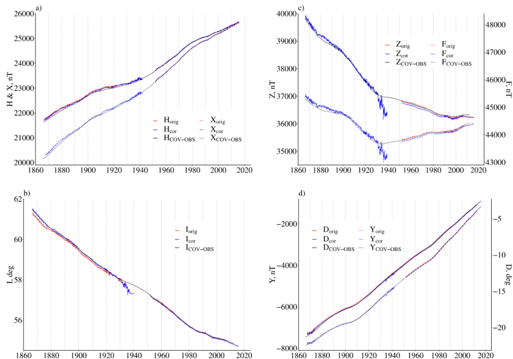
Figure 1: For the 1866 to 2015 time period, measured (red) and corrected (blue) series of the COI geomagnetic field elements (a) H and X; (b) I; (c) F and Z; (d) D and Y. The COV-OBS model predictions are in black.
