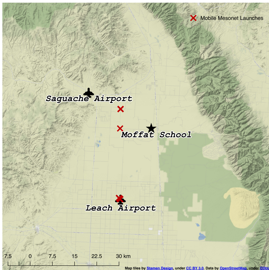
Figure 4. Sounding locations for the NSSL Mobile vehicle (red X's) and locations of profiling systems during LAPSE-RATE. The OU CLAMPS trailer performed all of their soundings at the Moffat School site. ©OpenStreetMap contributors 2020. Distributed under a Creative Commons BY-SA License
