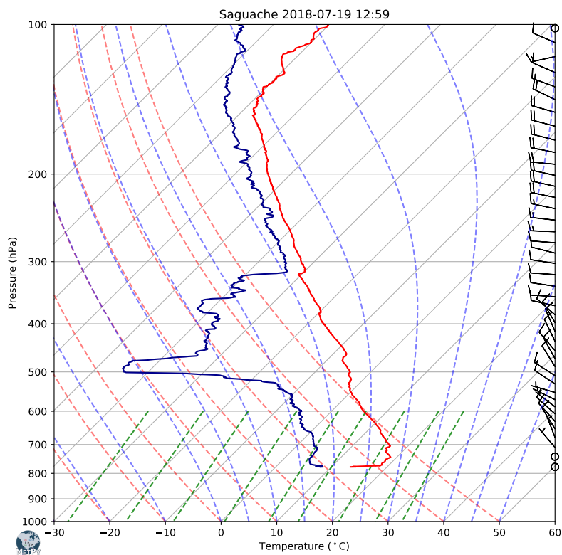
Figure 7. Sounding launched from near Saguache, CO at 1259 UTC. Image created using MetPy (May et al., 2008 - 2020).
