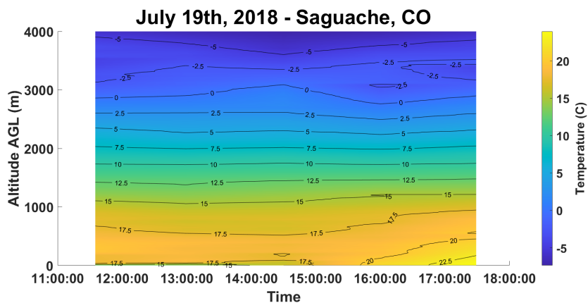
Figure 8. Time series of air temperature from 5 radiosondes launched near Saguache. Sounding times were 1135, 1259, 1430, 1600, and 1729 UTC. Temperature values between sounding times are interpolated.
