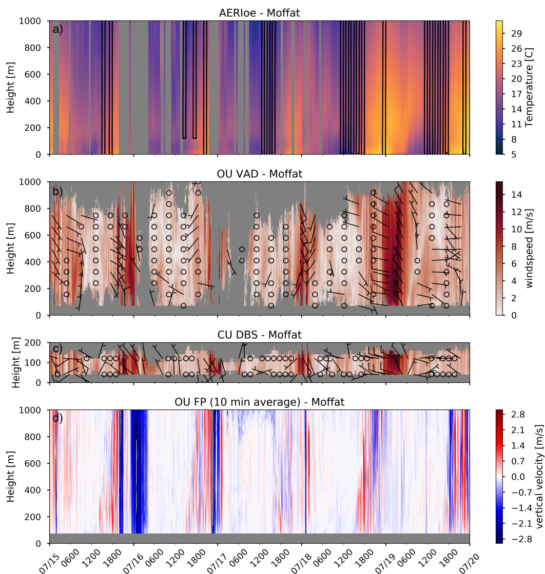
Figure 6. Time-height figures of temperature from the AERloe retrievals (a), wind speed and direction from the CLAMPS VAD (b), wind speed and direction from the CU DBS scan (c), and 10 minute averages of the vertical velocity measured from the CLAMPS vertical stare (d) from the full LAPSE-RATE campaign. All of these data were recorded at the Moffat site.
