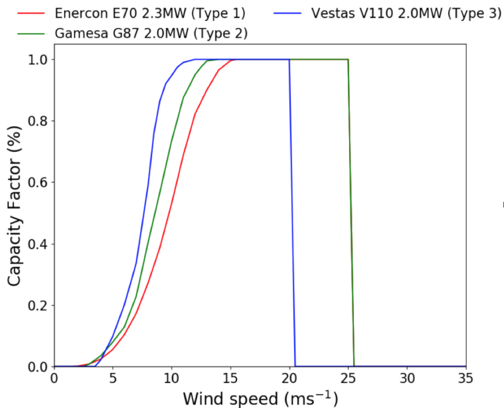
Figure B1. Wind power curves used in wind power model.
