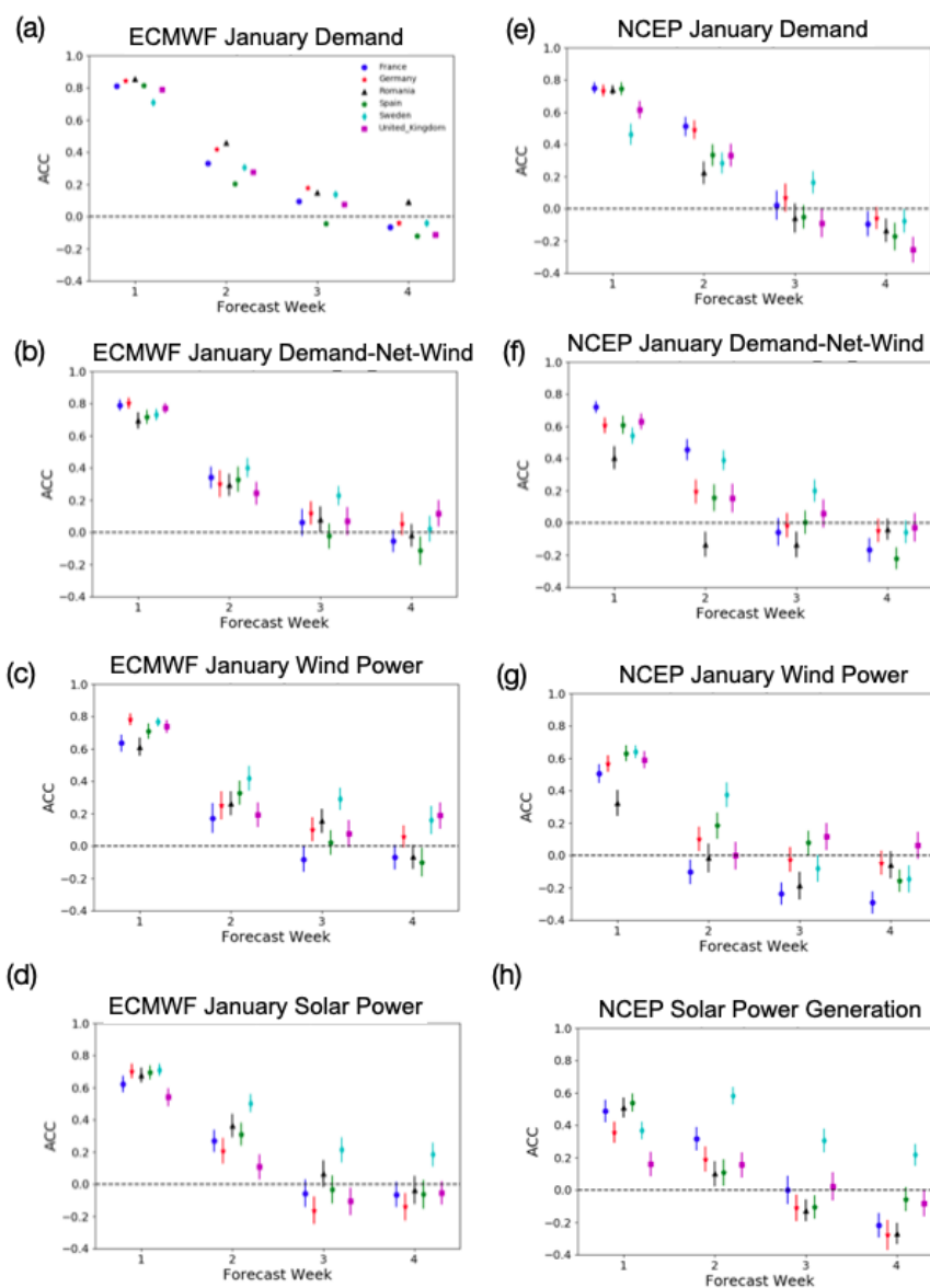
Figure 2. Forecasts of weekly-mean January energy-variables for the ECMWF (a-d) and NCEP (e-h) models. Definitions of the lead weeks are given in Section 2. Error bars show the 95% significance. Colours show a set of representative case study countries: France, Germany, Romania, Spain, Sweden and the United Kingdom
