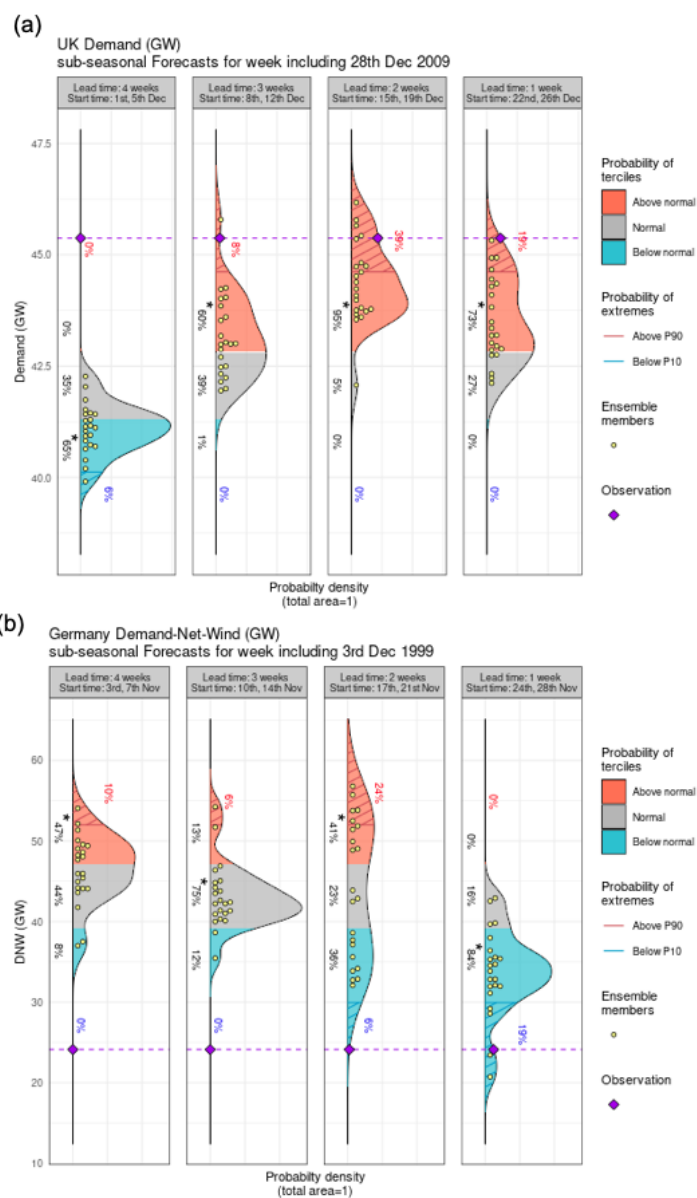
Figure 4. Weekly-mean forecasts verifying for the case study events of (a) UK high Demand, December 28th 2009 (b) Storm Anatol 2-8th December 1999. Purple dots give the weekly mean verification from ERA5. From left to right corresponds to forecasts launched from lead weeks 4 to 1. Definitions of the lead weeks are given in Section 2. Shaded areas represent climatological terciles with hatching showing the 10th and 90th percentiles calculated from 1979-2019 in ERA5.
