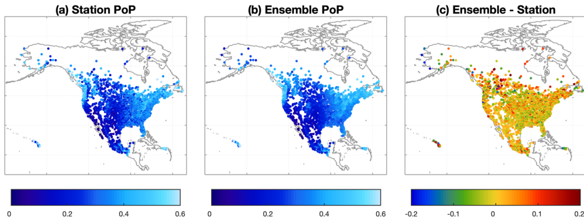
Figure 910. The probability of precipitation (PoP) from (a) station observations and (b) concurrent EMDNA ensemble estimates with their differences shown in (c). Stations with at least 5-year-long records from 1979 to 2018 are involved in the comparison.
