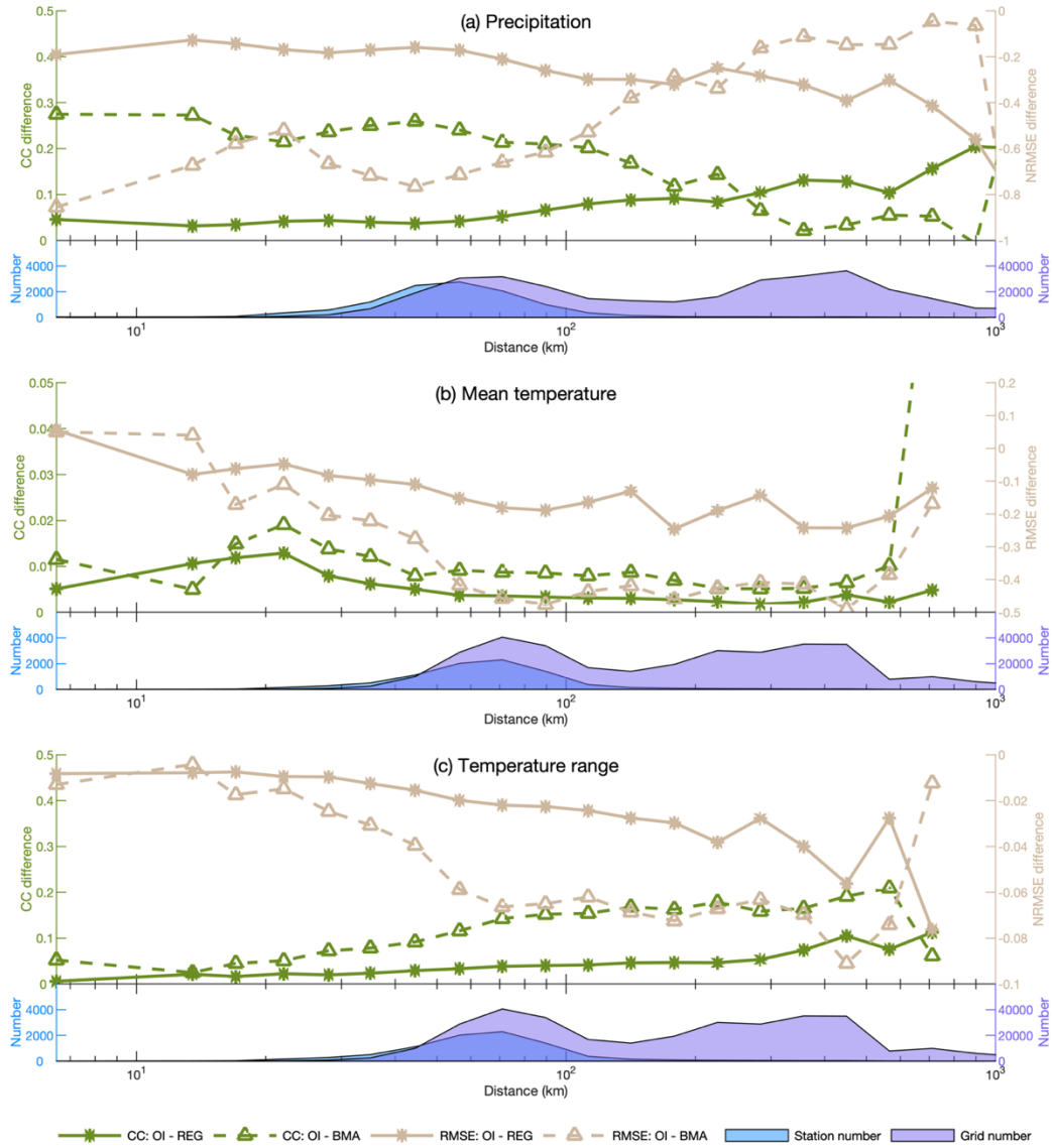
Figure 8. The improvement of OI-based station-reanalysis merged estimates against station-based regression (REG) and BMA merged reanalysis (BMA). The logarithmic X-axis shows the distance between the target station/grid and its 20th distant neighboring station. A larger distance represents a lower station density. The shaded area chart shows the numbers of stations and grid points corresponding to the same distance, which is the same for mean temperature and temperature range.
