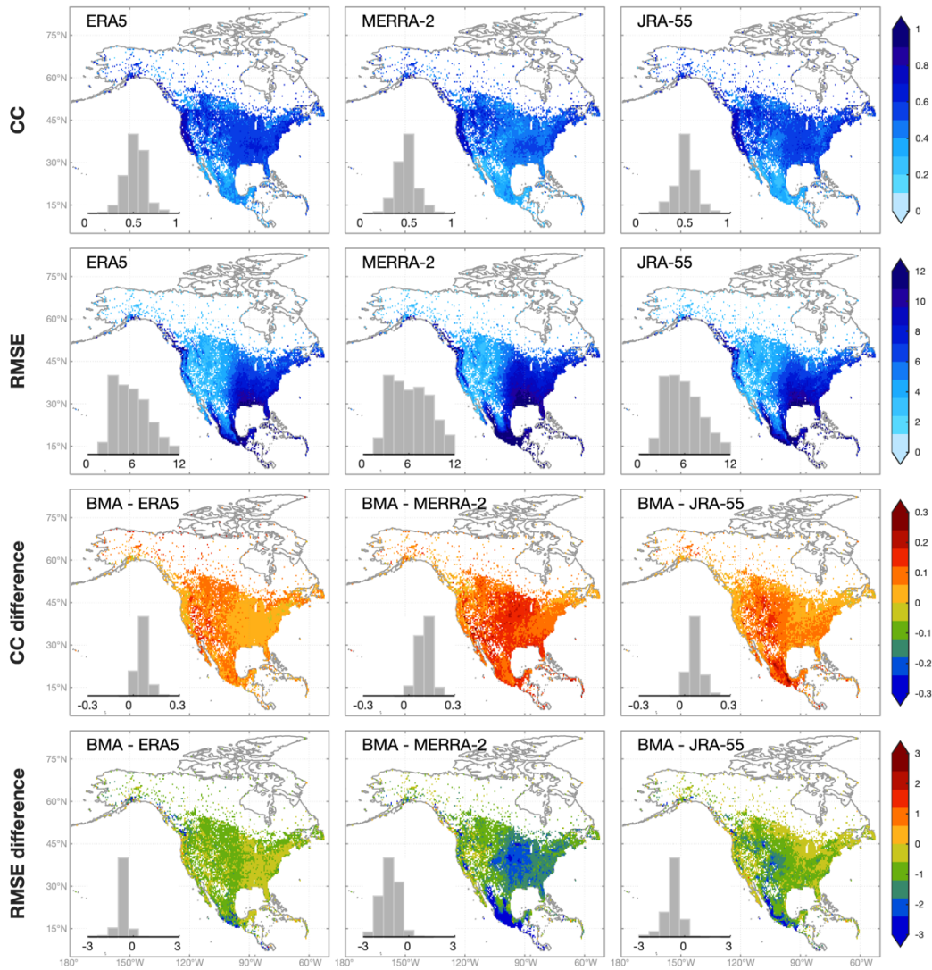
Figure 3. The spatial distributions and histograms of CC (the first row) and \sqrt{\text{RMSE}} (the second row) based on raw reanalysis precipitation estimates (ERA5, MERRA-2, and JRA-55). The improvement of BMA-merged estimates against raw reanalysis estimates is shown in the third and fourth rows. The maps are at the 0.5^\circ resolution, and the value of \sqrt{\text{RMSE}} for each 0.5^\circ grid point, \sqrt{\text{RMSE}} is the median metric of median value of all stations located within the grid is shown.
