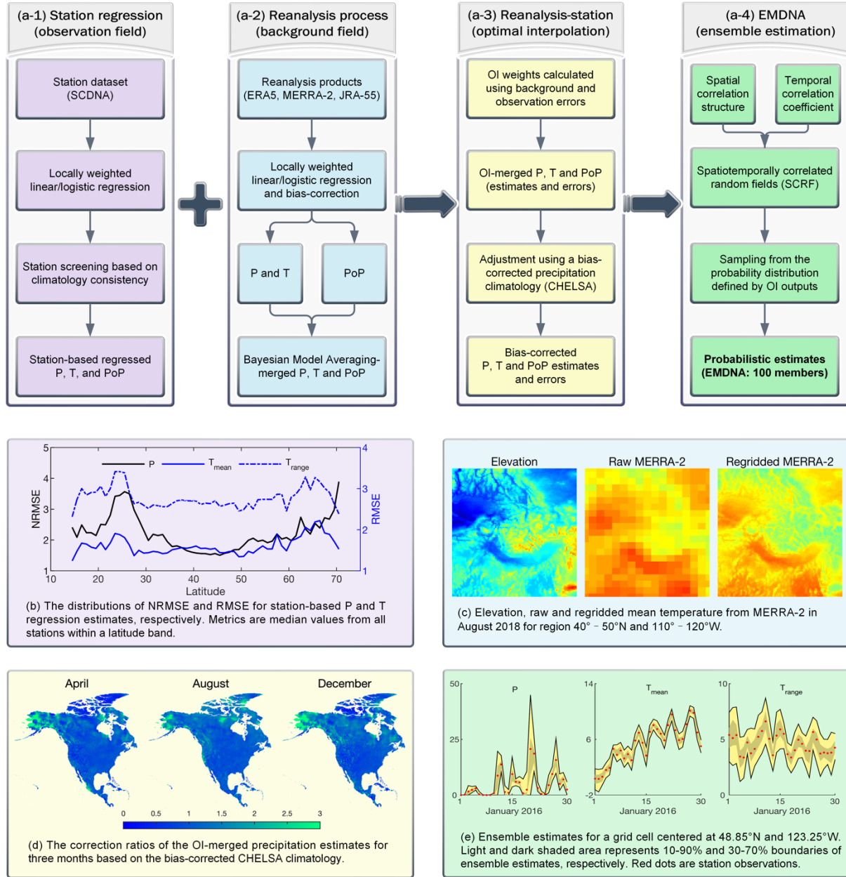
Figure 2. (a) The flowchart outlining the main steps for producing EMDNA. P represents precipitation and T represents temperature. (b-e) demonstrate output examples from (a-1 to -4), respectively. (b) Latitudinal distribution of the root mean square error (RMSE) for temperature and normalized RMSE (NRMSE) for precipitation (Sect. 3.1). (c) Example showing the mean temperature of MERRA-2 before and after regridding (Sect. 3.2). (d) The correction ratios calculated using precipitation climatology from the bias-corrected CHELSA (Sect. 3.3). (e) Example of the ensemble-based distributions of precipitation and temperature estimates from EMDNA (Sect. 3.4).
