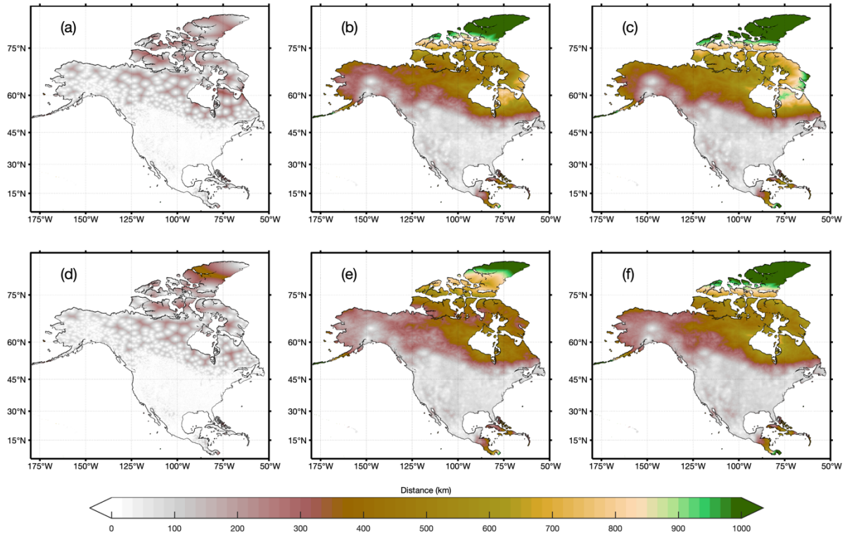
Figure 1. The color of each 0.1^\circ grid indicates the radial radius to find (a) one, (b) 20, and (c) 30 neighboring stations for precipitation (a-c) and temperature (d-f).
