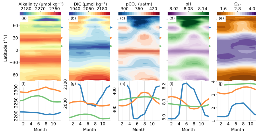
Figure 11. Hovmoeller plots (a-e) showing the zonally averaged seasonal climatologies for (a) total alkalinity, (b) dissolved inorganic carbon, (c) p\text{CO}_2 , (d) pH, and (e) aragonite saturation state ( \Omega_{Ar} ). The second row of panels (f-j) show the corresponding variables for a high (55°N, 180°E, blue), mid (30°N, 180°E, orange) and low-latitude (10°N, 180°E, green) location. The units for (f-j) correspond with the units in (a-e).
