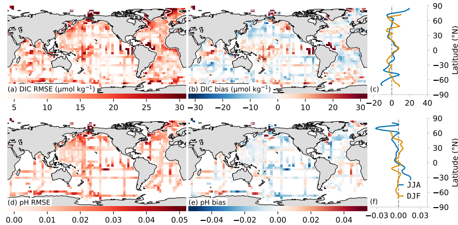
Figure 5. Root mean squared error (RMSE - a,d) and biases (b,c,e,f) for: dissolved inorganic carbon (DIC, top) and pH (bottom) compared with in situ GLODAP v2.2019 data. The two subplots in the right most column compare the zonally-averaged bias for JJA and DJF. Data were processed for plotting as described in Section 4.
