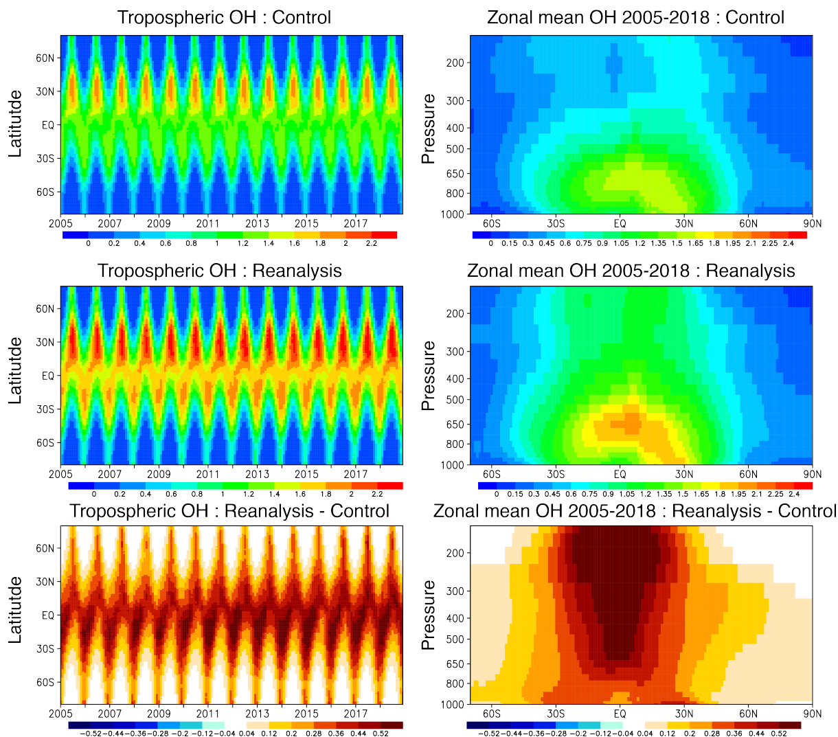
Figure 9. Latitude-pressure cross section of the mean OH concentration (right panels) averaged during 2005-2018 and time-latitude cross-section of the monthly mean OH concentration averaged between the surface and 300 hPa (left panels). The mean OH concentrations from the control run (upper row), reanalysis (center row) and the difference between the reanalysis and the model simulations (lower row) are shown. Units are 10^6 molecules \text{cm}^{-3} .
