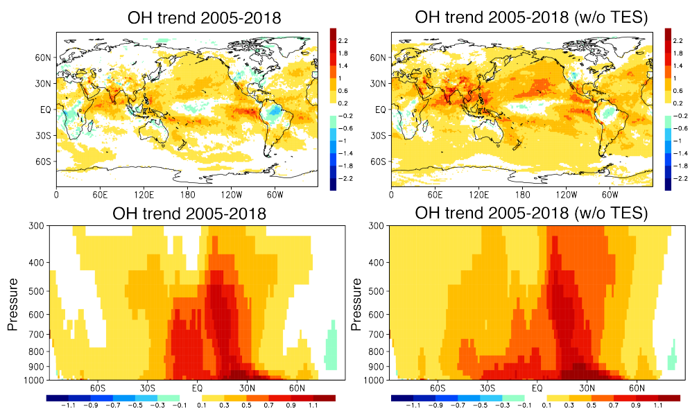
Figure 17. Same as in Fig. 16, but for tropospheric OH (in 10^6 molecules \text{cm}^{-3} per year, upper row) and the latitude-pressure cross-section of OH trends (in % per year, lower row) for the years 2005-2018.
