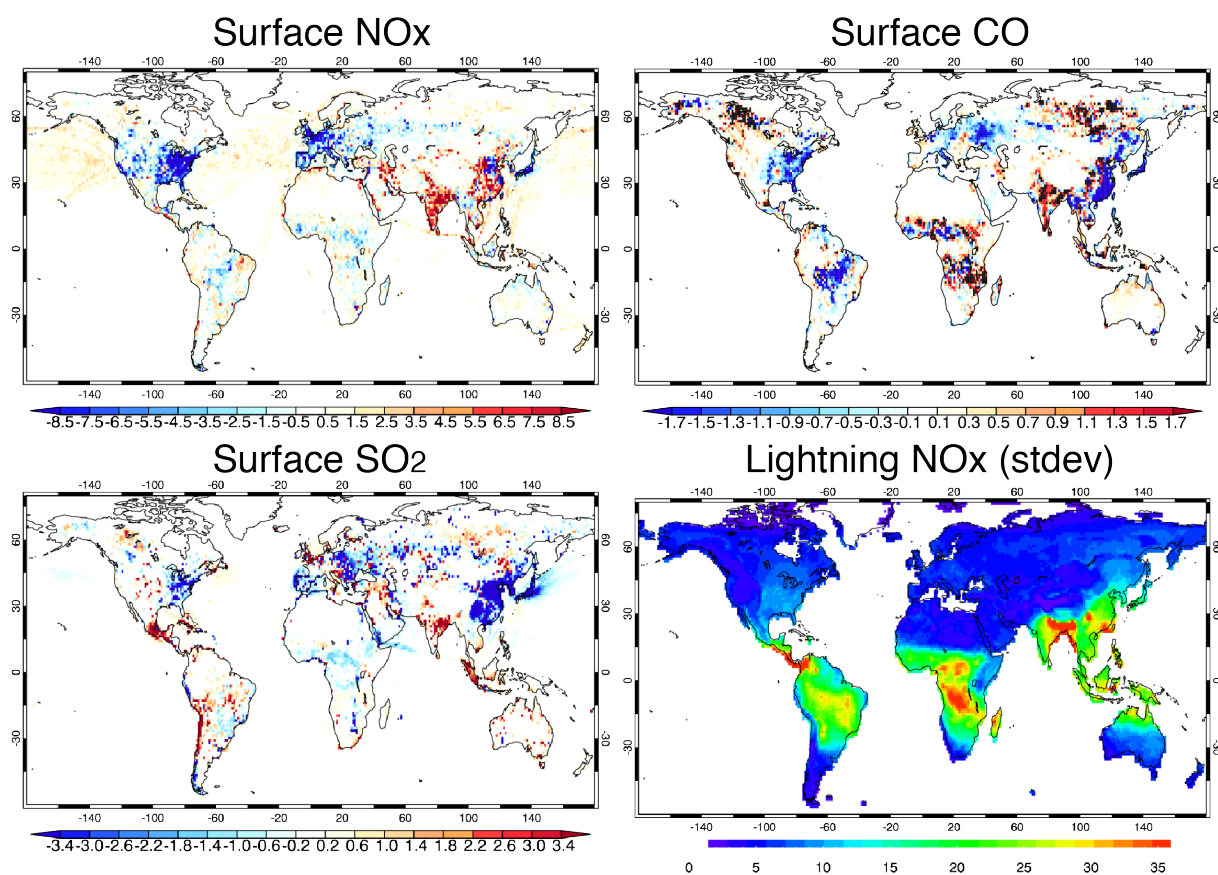
Figure 14. Global distribution of linear trend of the a posteriori surface \text{NO}_x emissions (in 10^{-13}\text{kgNm}^{-2}\text{s}^{-1} per year), surface CO emissions (in 10^{-11}\text{kgCOm}^{-2}\text{s}^{-1} per year), and surface \text{SO}_2 emissions (in 10^{-14}\text{kgSm}^{-2}\text{s}^{-1} per year), and standard deviation of the a posteriori lightning \text{NO}_x emissions (in 10^{-14}\text{kgNm}^{-2}\text{s}^{-1} per year) for the period 2005–2018. The red (blue) colour indicates positive (negative) trends.
