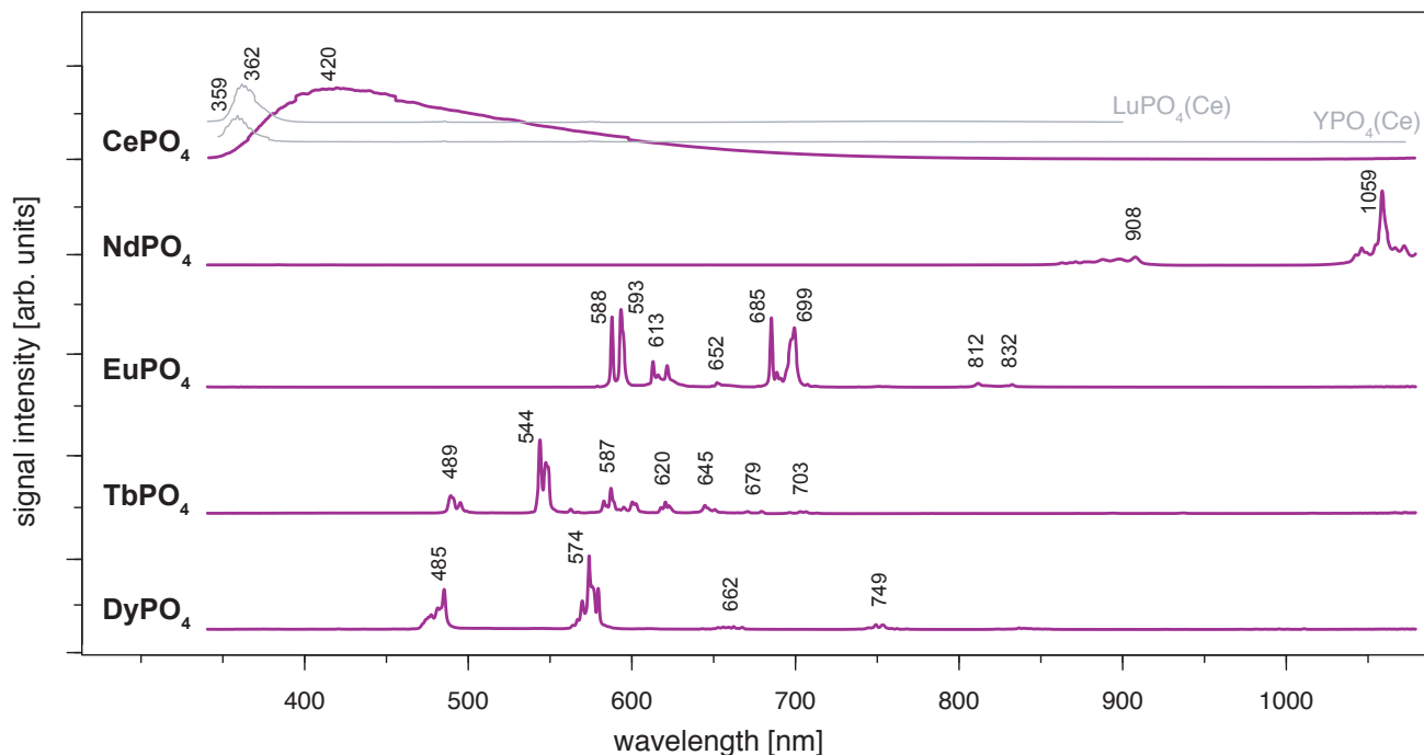
Figure 4. LiF reference spectra obtained with 325 nm laser excitation depict the diagnostic emission lines for the REE phosphates NdPO 4 , EuPO 4 , TbPO 4 , and DyPO 4 (given values represent wavelength of most intense emission in nm for each transition, cf. Tab. 2). CePO 4 is included for completeness, diagnostic emissions are shown by the grey lines representing spectra from two non-luminescent REE PO 4 samples with Cerium contaminations (see further explanation in the text along with Cerium concentrations in those samples based on neutron activation analysis (NAA) results)
